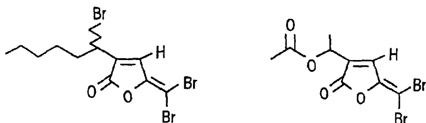
FURANONE 34
