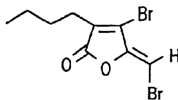
FURANONE 2
