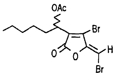
FURANONE 36
