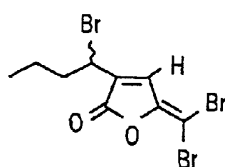
FURANONE 27
