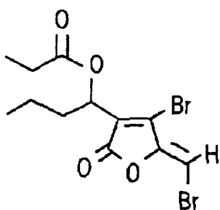
FURANONE 46
