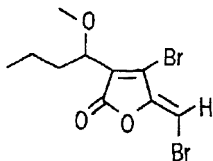
FURANONE 50
