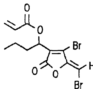
FURANONE 43
