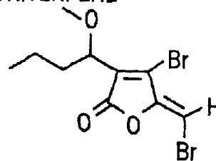
FURANONE 53
