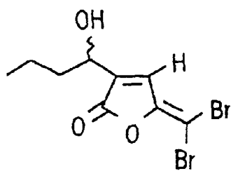
FURANONE 38
