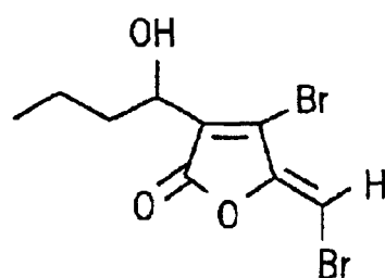
FURANONE 4
