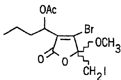
FURANONE 6
