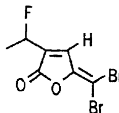
FURANONE 60
