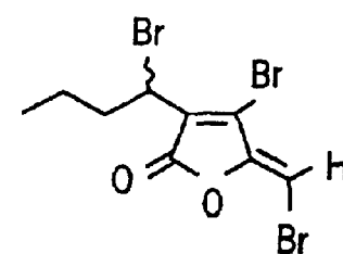
FURANONE 26
