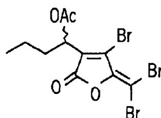
FURANONE 21
