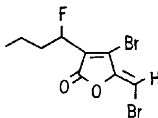
FURANONE 45
