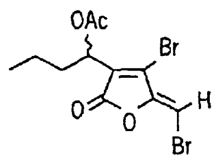
FURANONE 22
