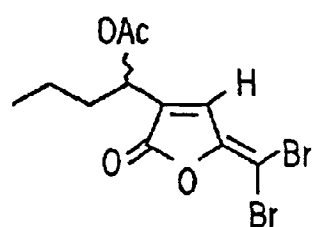
FURANONE 23
