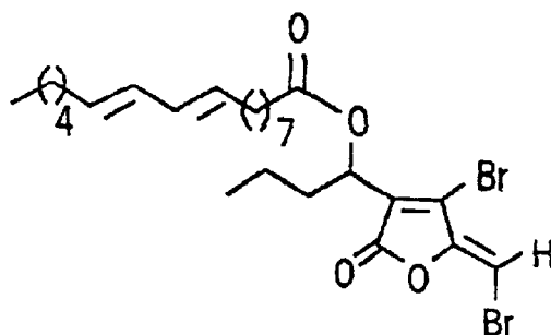
FURANONE 54
