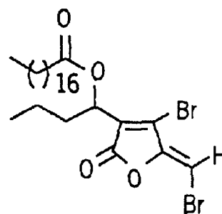
FURANONE 41
