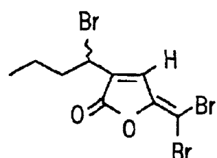
FURANONE 25
