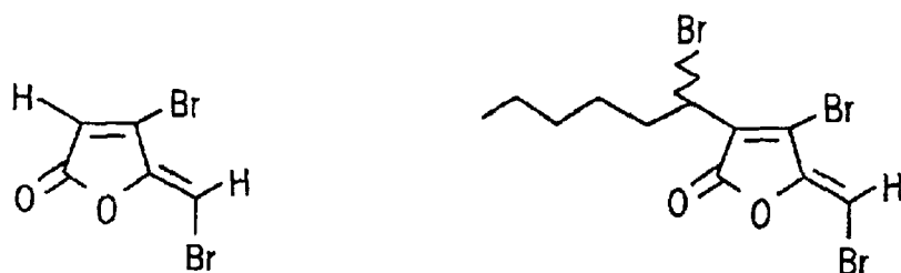
FURANONE 30
