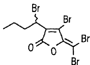
FURANONE 20
