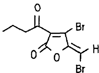
FURANONE 42
