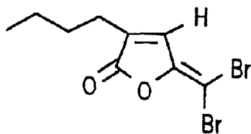
FURANONE 8
