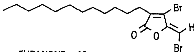
FURANONE 19
