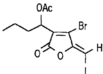
FURANONE 5
