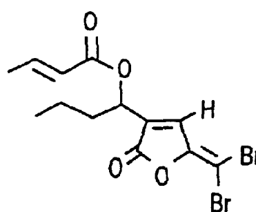
FURANONE 49
