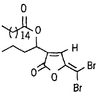
FURANONE 40
