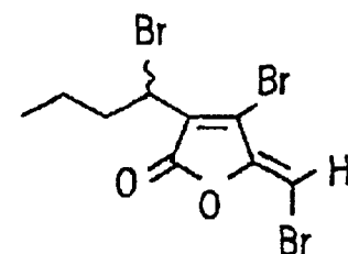
FURANONE 24
