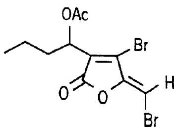
FURANONE 3
