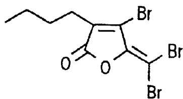
FURANONE 1
