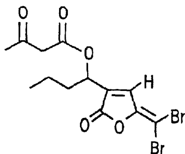
FURANONE 52
