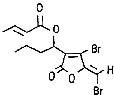
FURANONE 48
