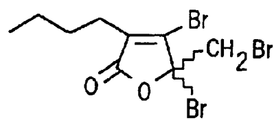
FURANONE 9
