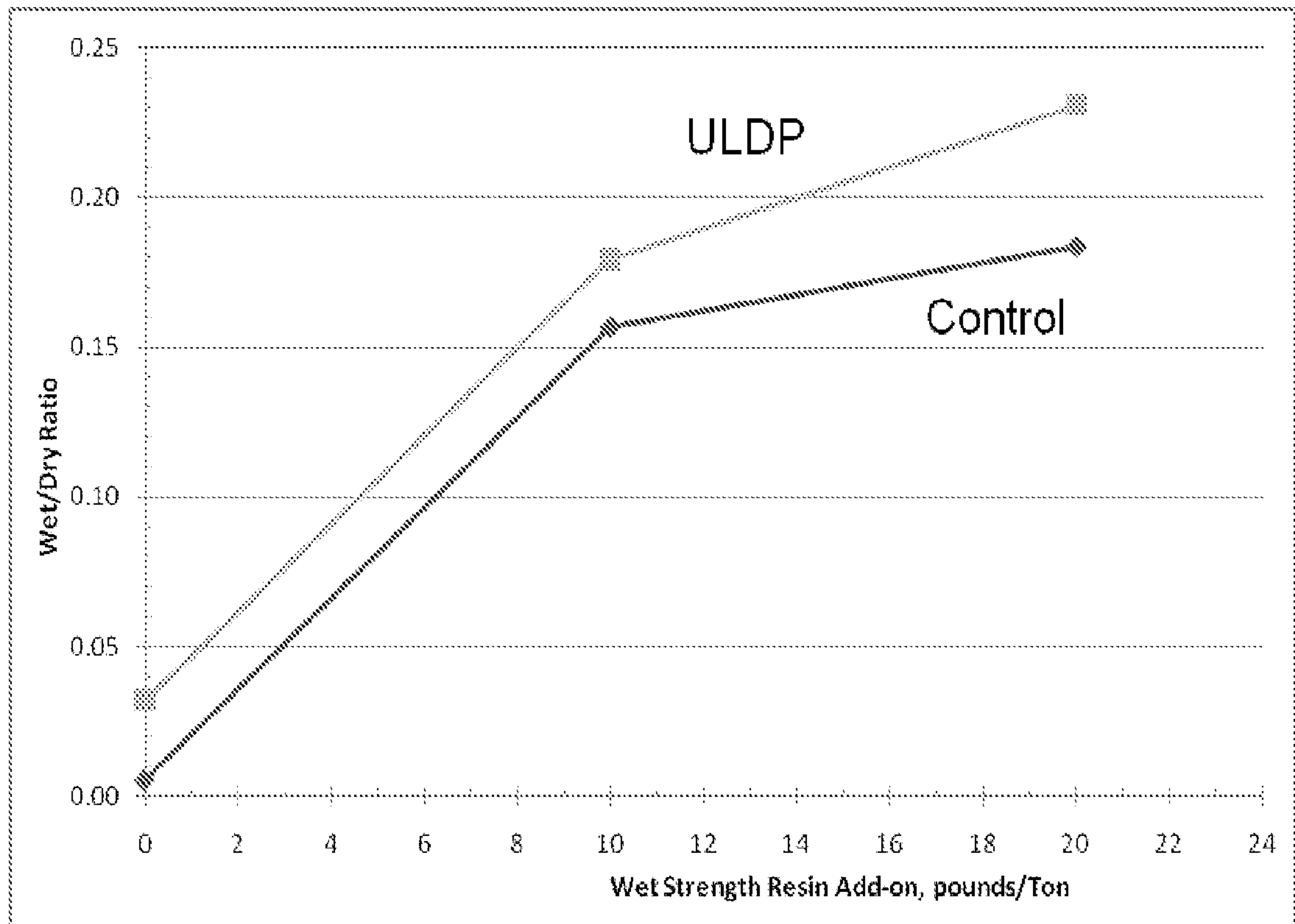
Figure 2. Wet/Dry strength ratio given as a function of wet strength resin level.
