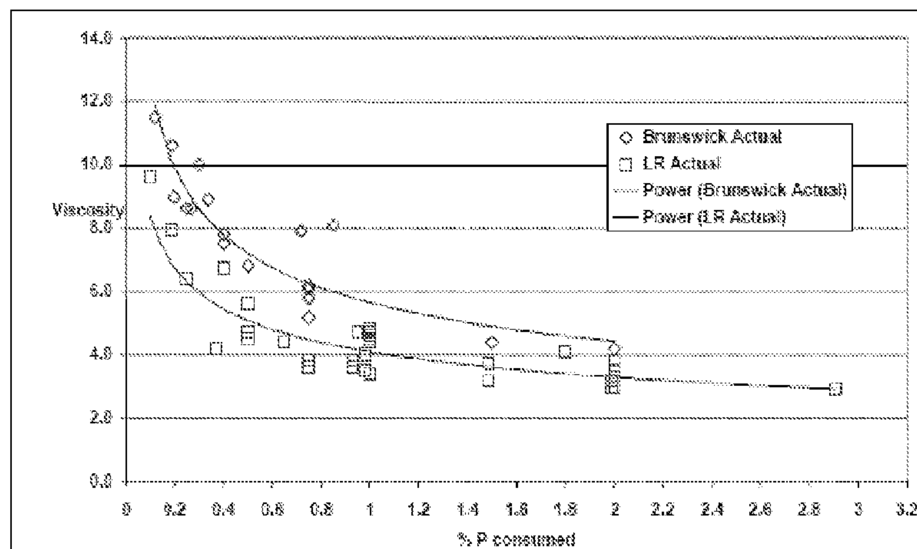
Final 0.5% Capillary CED viscosity as a function of % peroxide (based on pulp) consumed.
