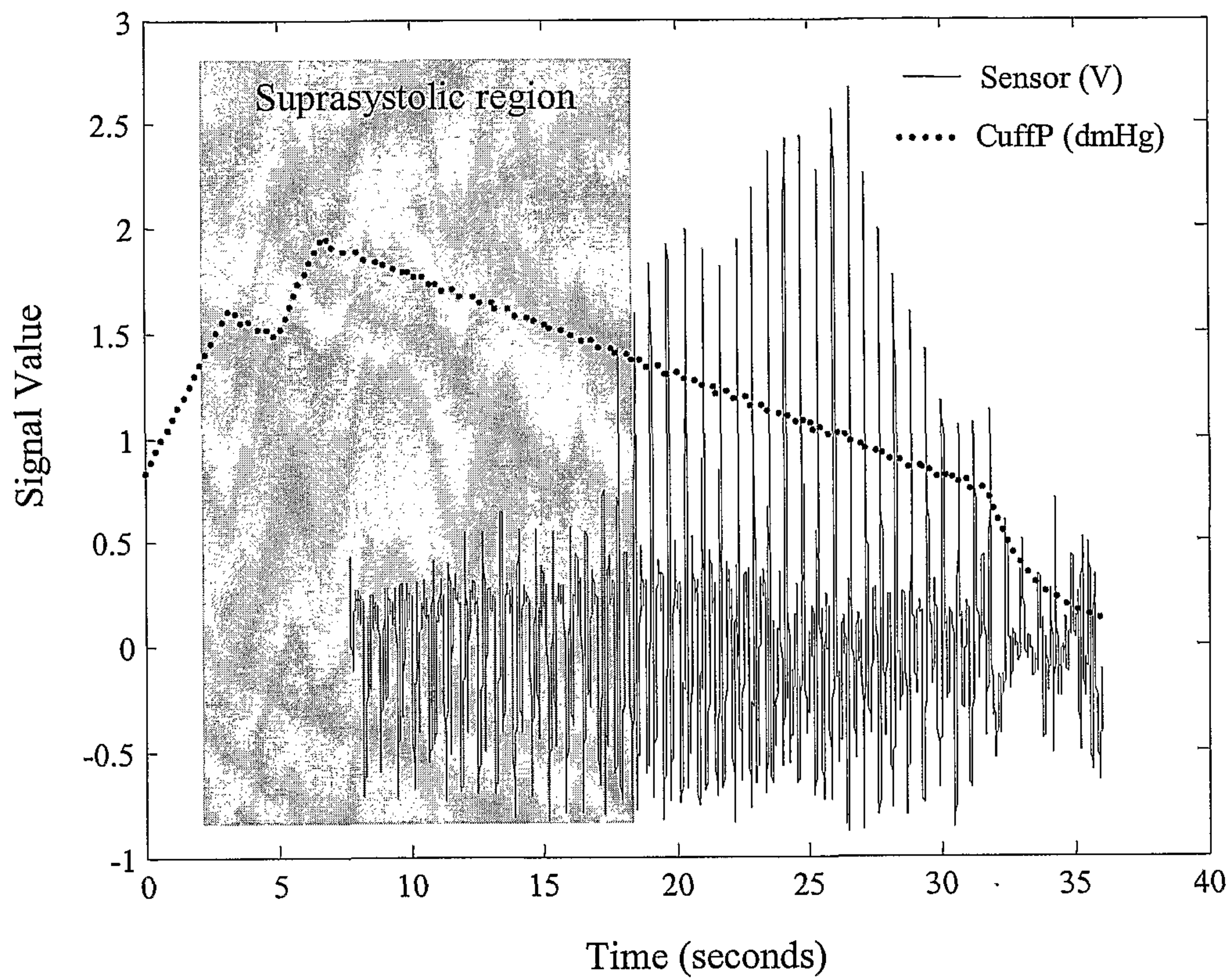
Figure 1: Typical signal from piezoelectric sensor
