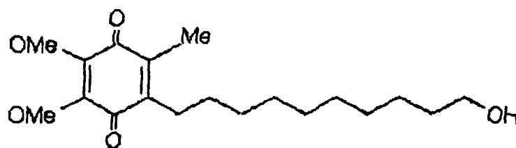
2,3-dimethoxy-5-methyl-6-(10-hydroxydecyl)-1,4-benzoquinone, idebenone
