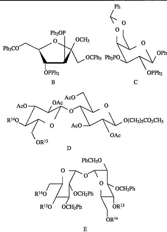
Asymmetric Hydrocyanation Using Ligands (L) B-E
