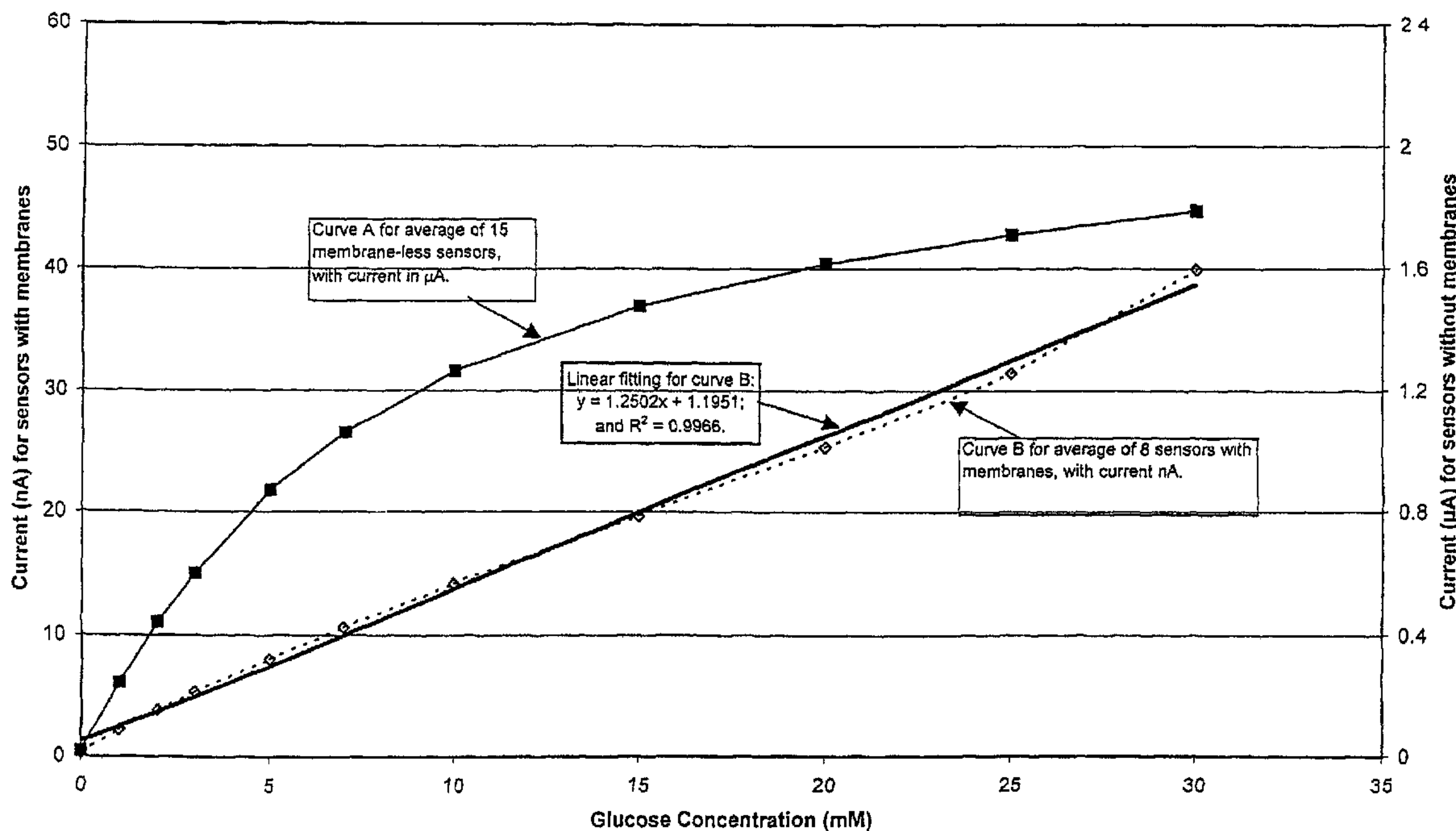
Calibration Curves at 37 °C
