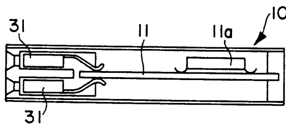
FIG. 2 (PRIOR ART)
