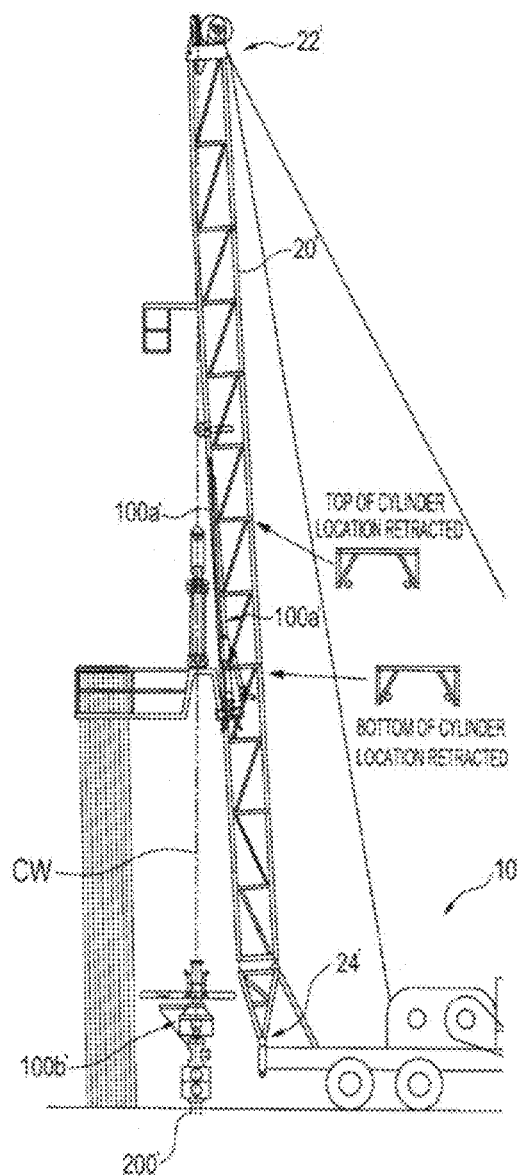
FIG. 2 PRIOR ART
