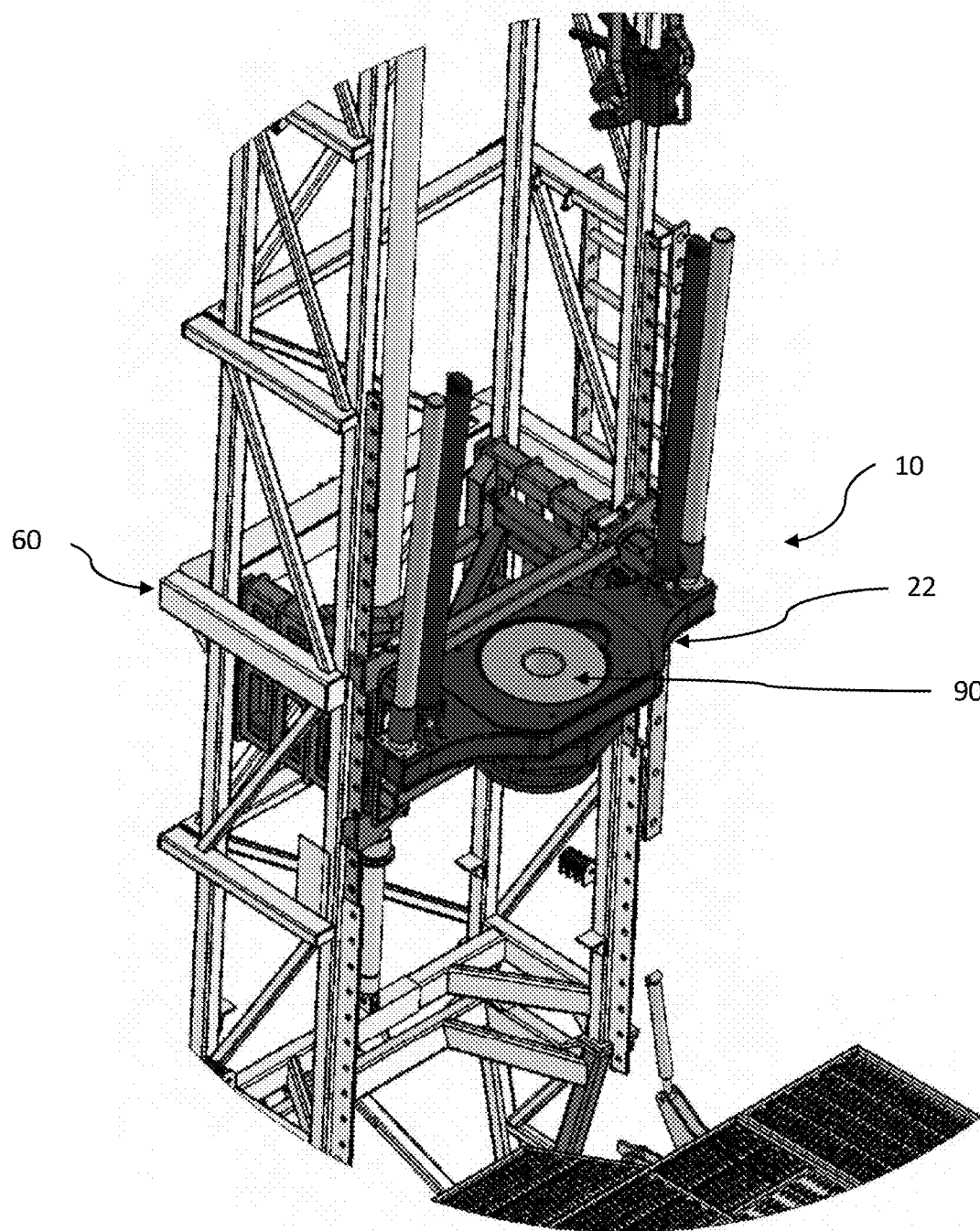
DETAIL A
