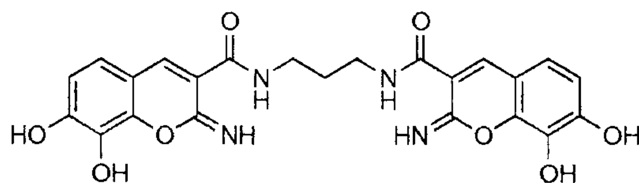
Structure of iminodyn-22.
