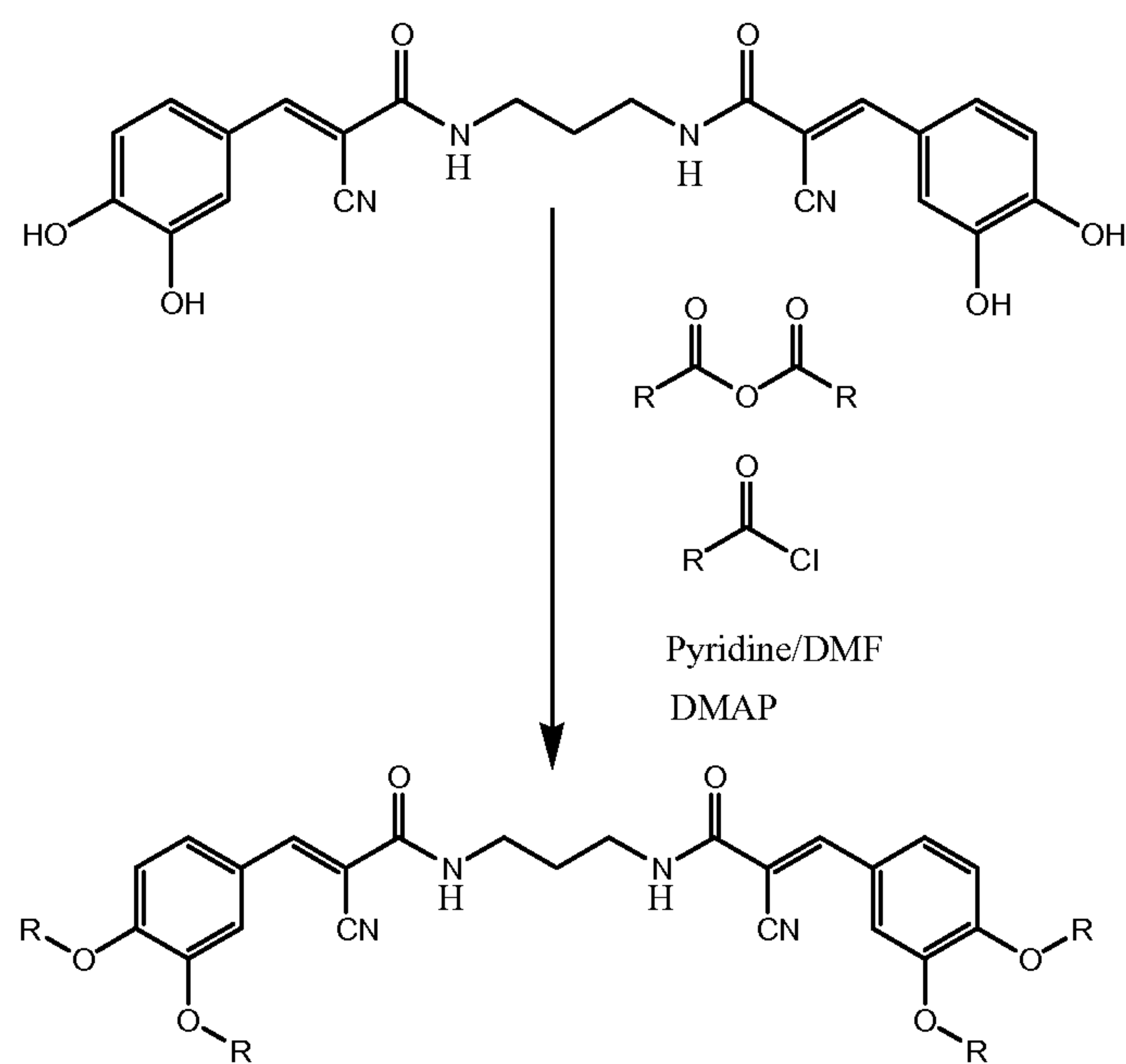
Scheme 3: Synthesis of prodrugs
