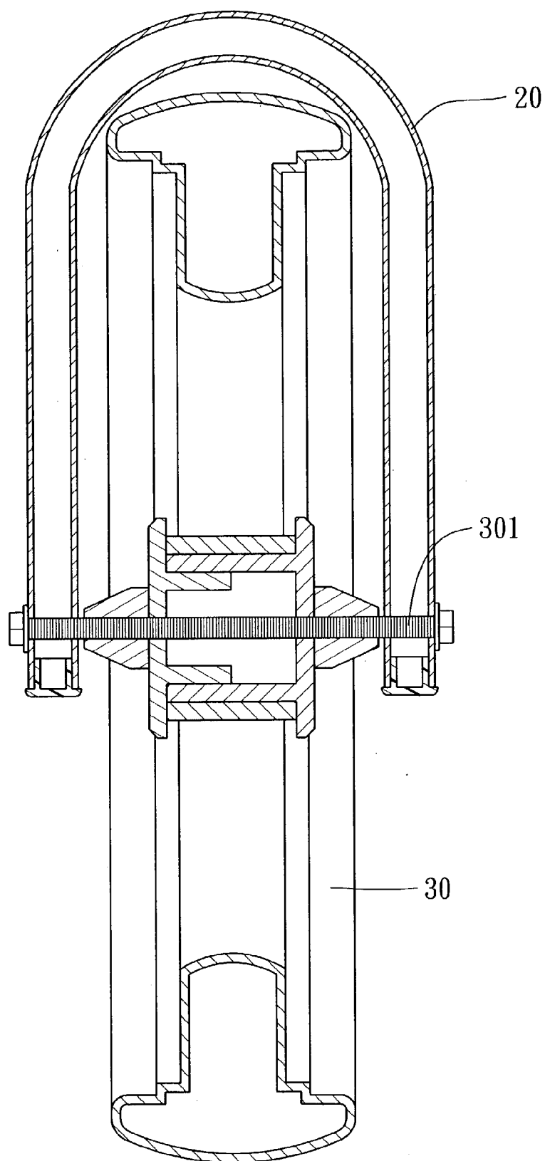
FIG. 2 (PRIOR ART)
