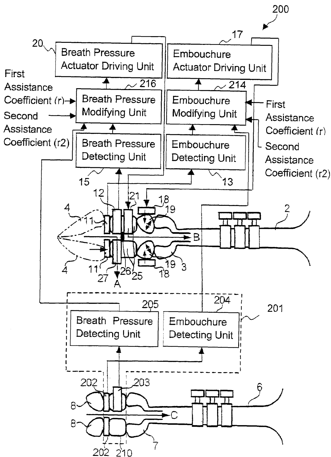
Fig. 3 Configuration of Assisting Apparatus
