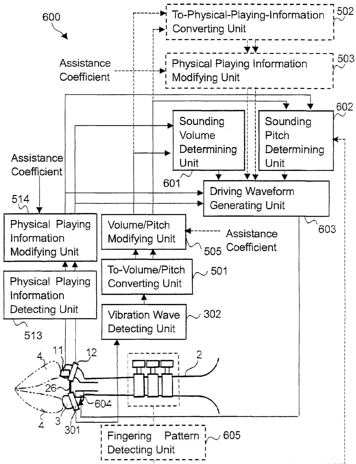
Fig.9 Configuration of Assisting Apparatus
