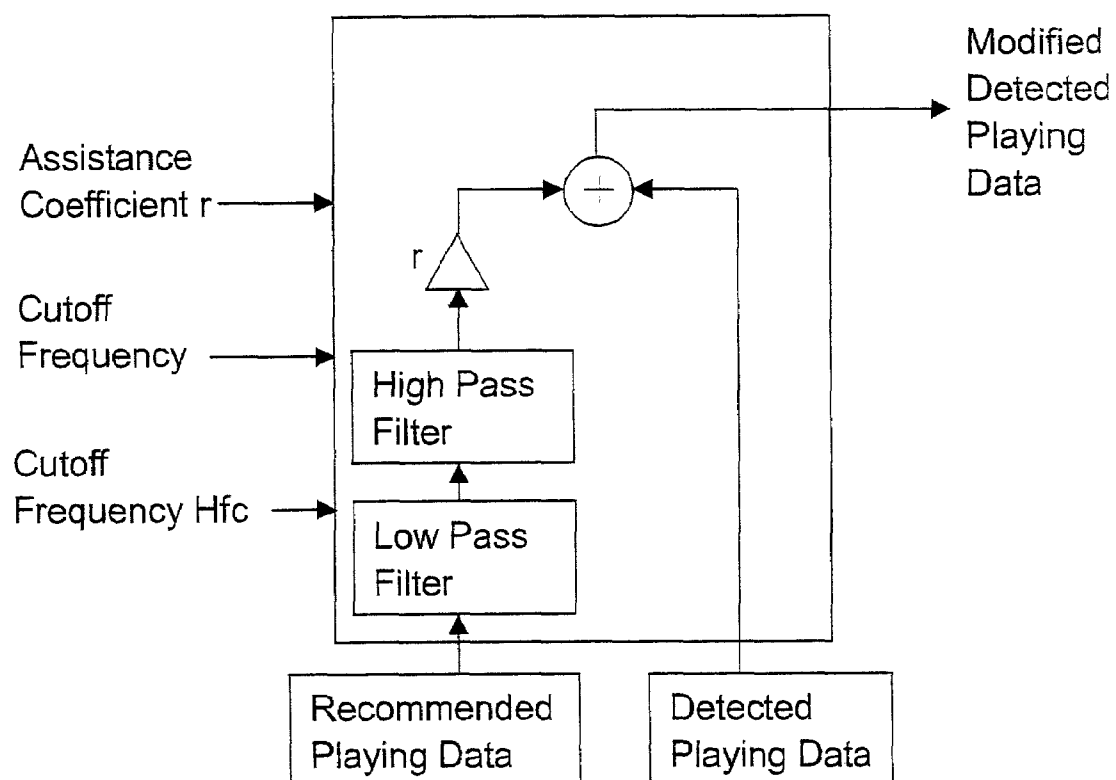
Fig. 16 Circuit Diagram of Modifying Unit and Data Processing
