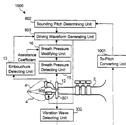
Configuration of Assisting Apparatus
