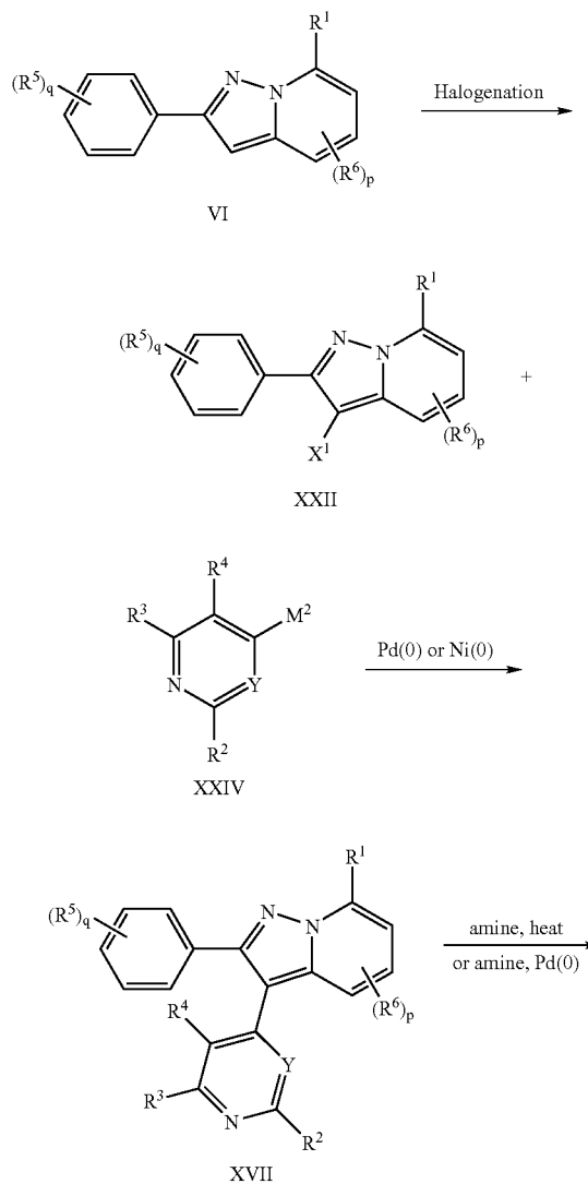
Scheme 4
