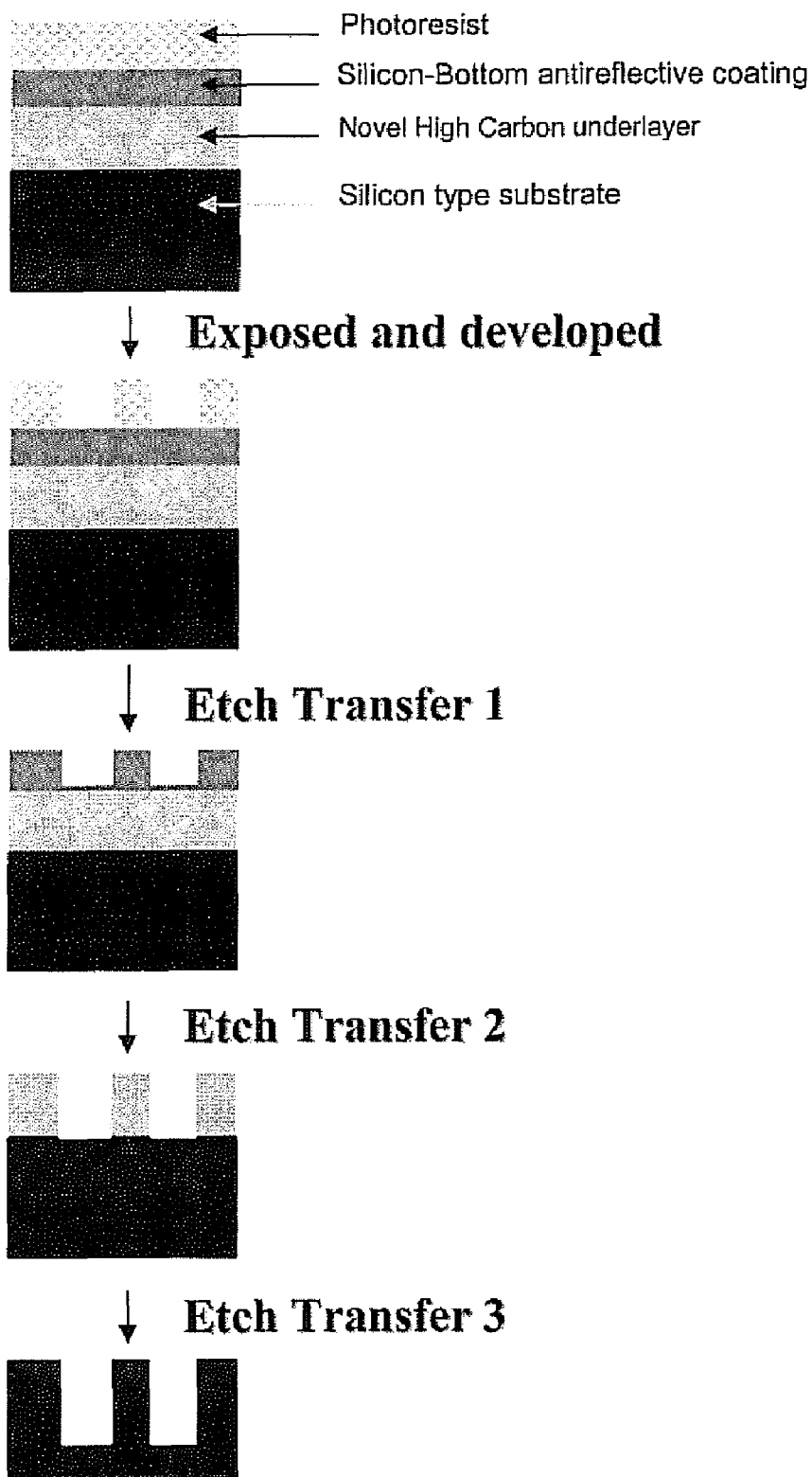
Figure 3: Imaging Process of a Trilayer
