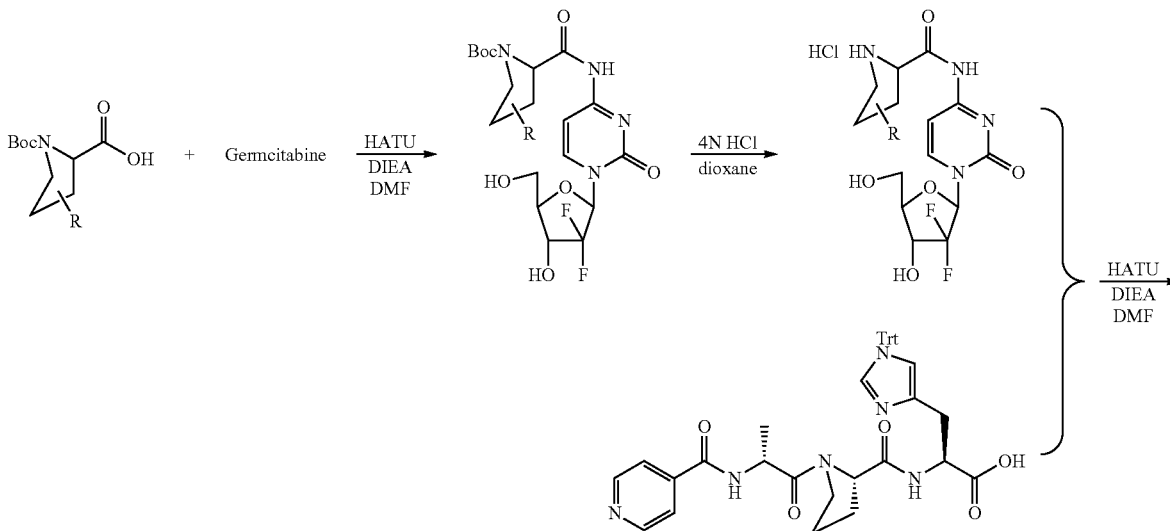
Scheme 1: General synthetic route to 4735 analogues
