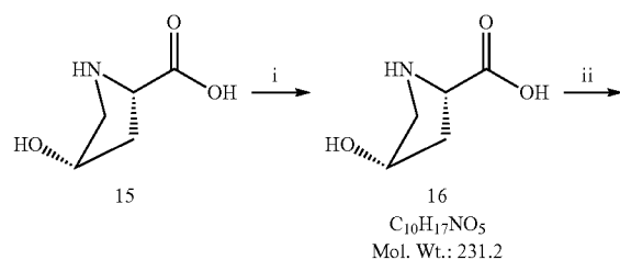
Scheme 3: Synthetic route to substituted Proline analogues
