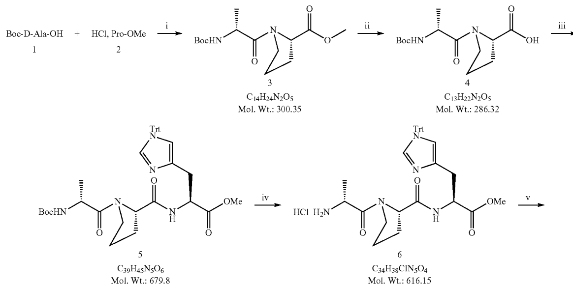
Scheme 2: Synthetic route 4735D
