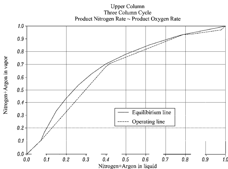
FIG. 1 (Prior Art)
