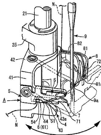
ENLARGED PART β
