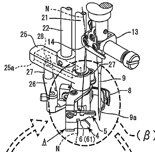
ENLARGED PART \alpha
