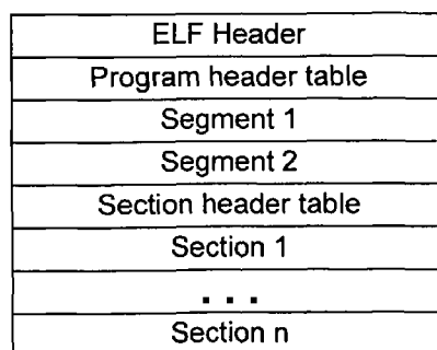
ELF File Structure
