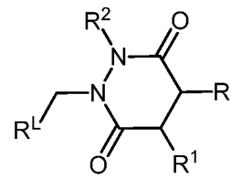
(VI-h)
