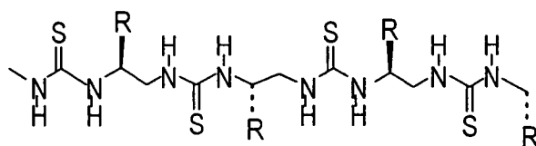
Polythioureas
