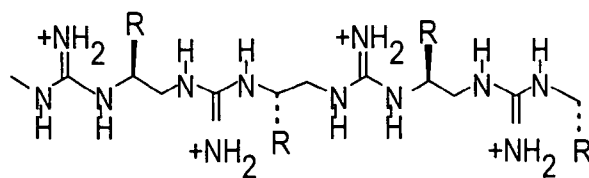
Polyguanidiniums
