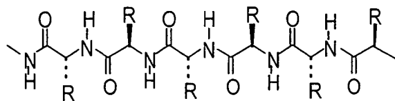
Peptides
