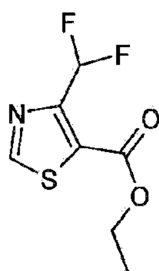
b) Preparation of Intermediate (1c)
