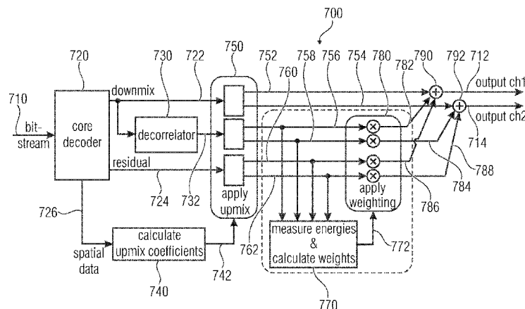
FLOW DIAGRAM OF DECODER
