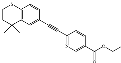
(Tazarotene)
