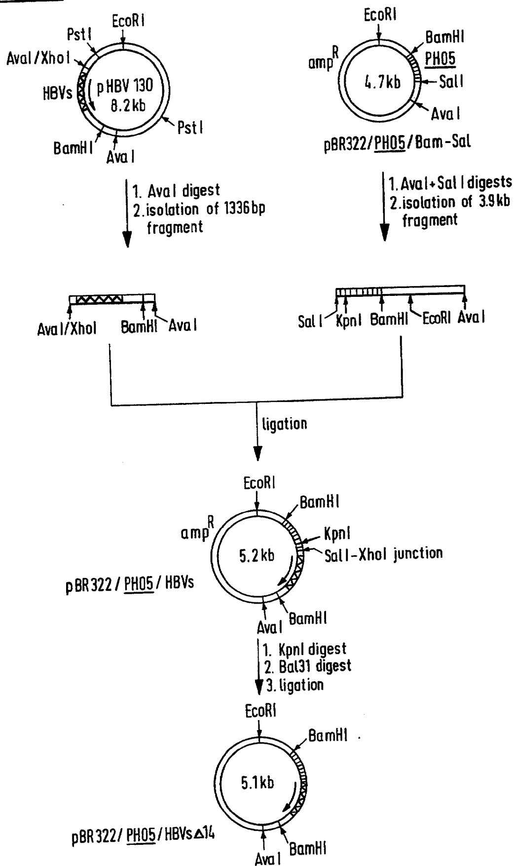
Fig. 24 CONSTRUCTION OF A CORRECT PH05-HBV s JUNCTION
