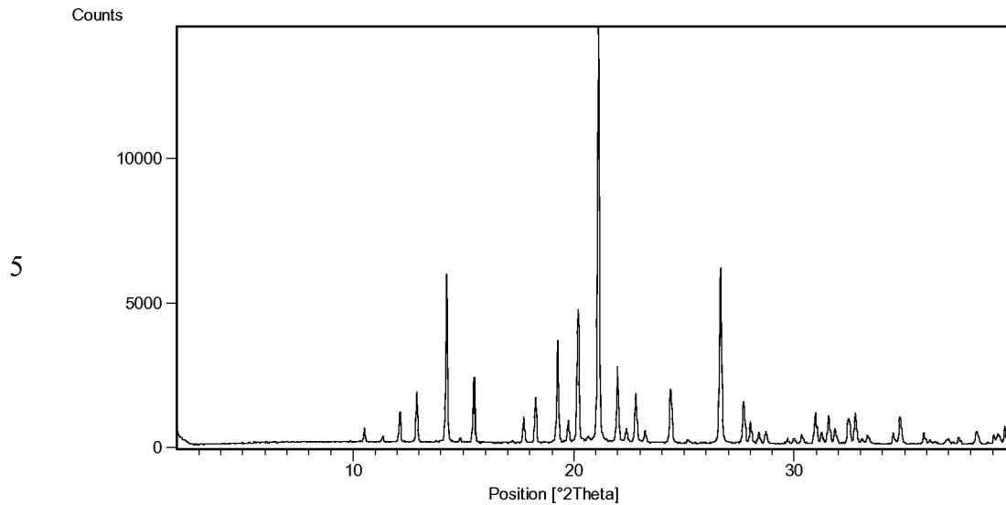
(XRPD pattern 1).
