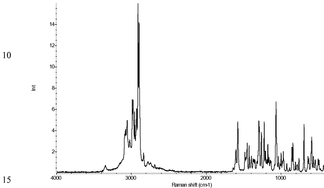
Raman spectrum (1).
