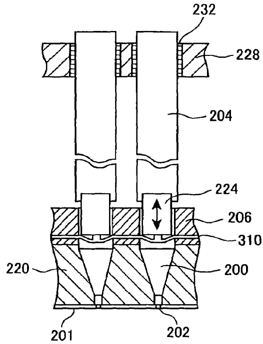
FIG. 1 RELATED ART
