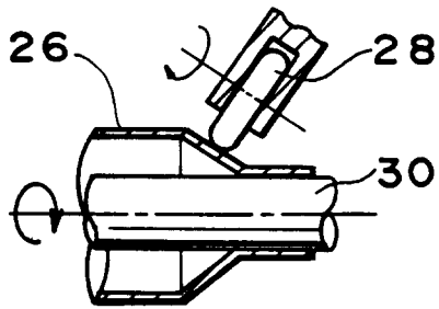
FIG. 5 (PRIOR ART)
