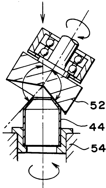
FIG 10 (PRIOR ART)
