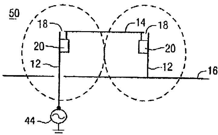
FIG. 5 PRIOR ART
