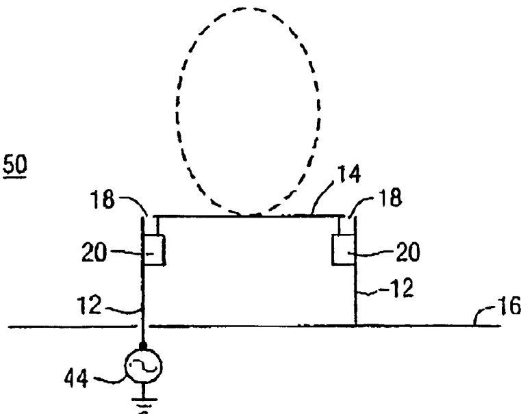
FIG. 7 PRIOR ART
