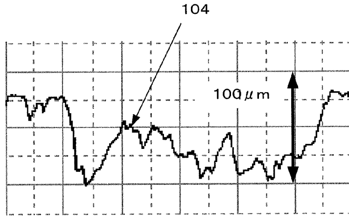
<MACHINED SURFACE ROUGHNESS UNDER CONVENTIONAL CONDITIONS 75 μ mRz>
