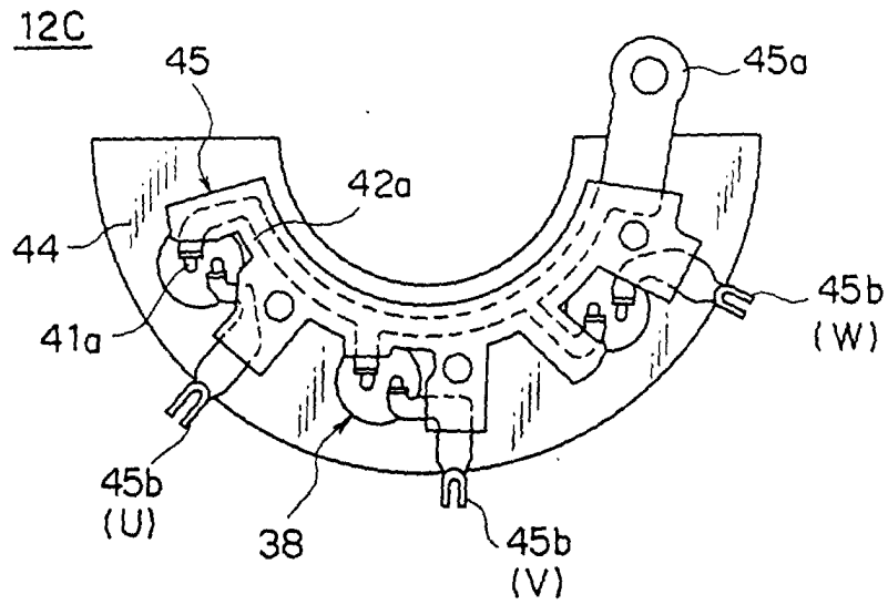
FIG. 32 PRIOR ART
