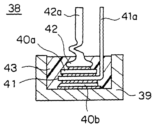
FIG. 33 PRIOR ART
