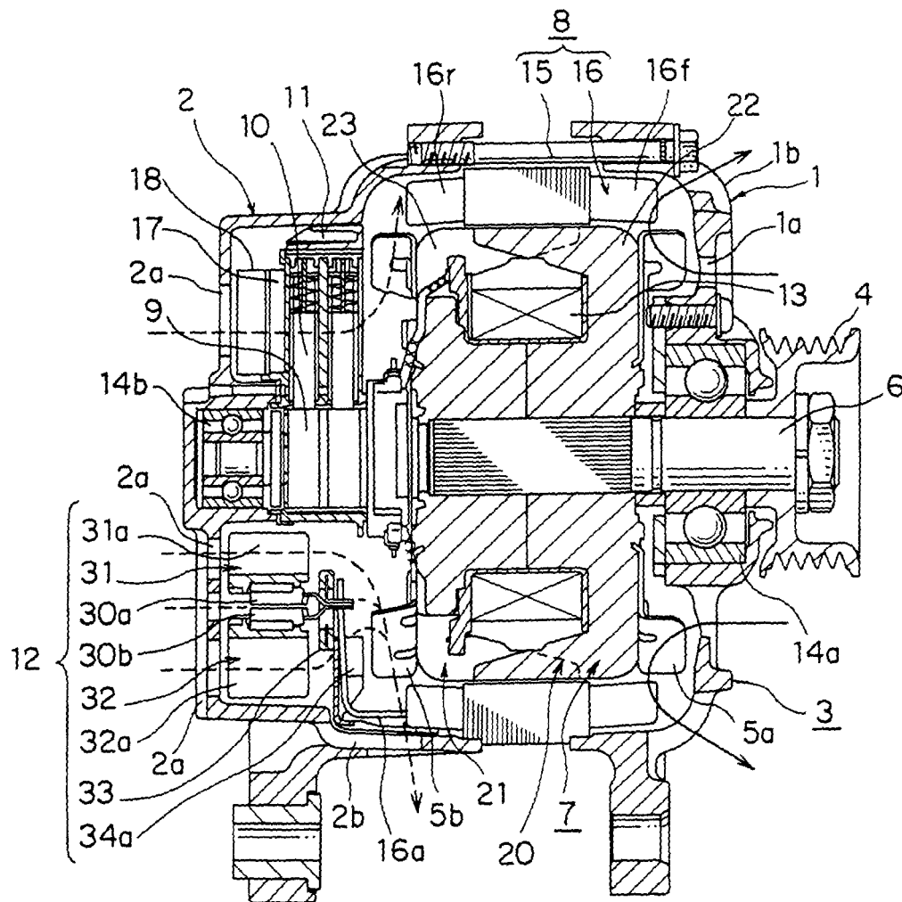
FIG. 21 PRIOR ART
