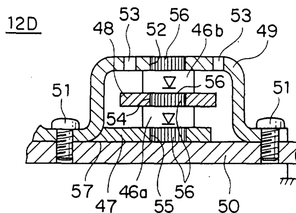
FIG. 34 PRIOR ART
