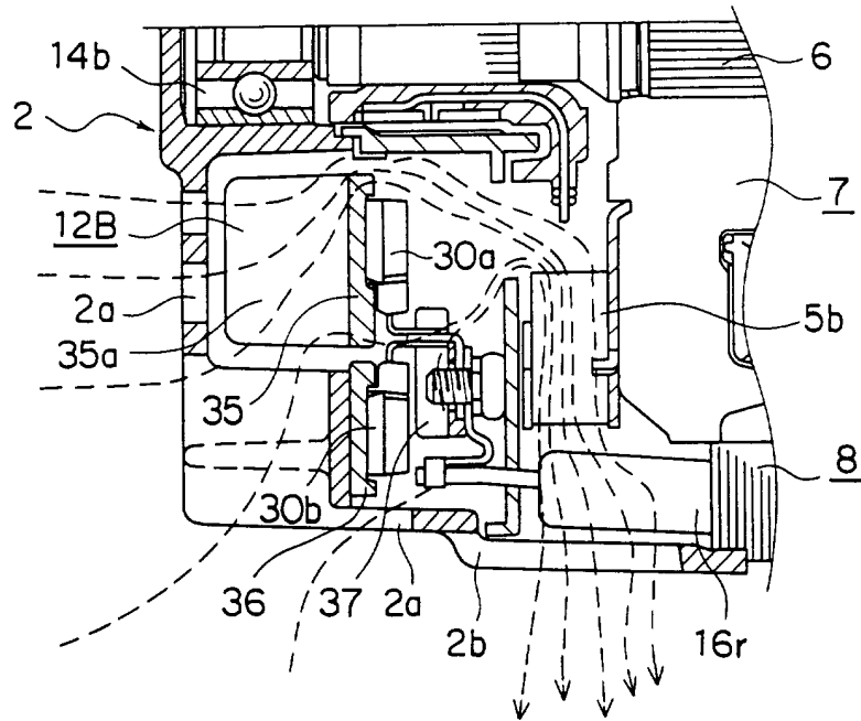
FIG. 31 PRIOR ART
