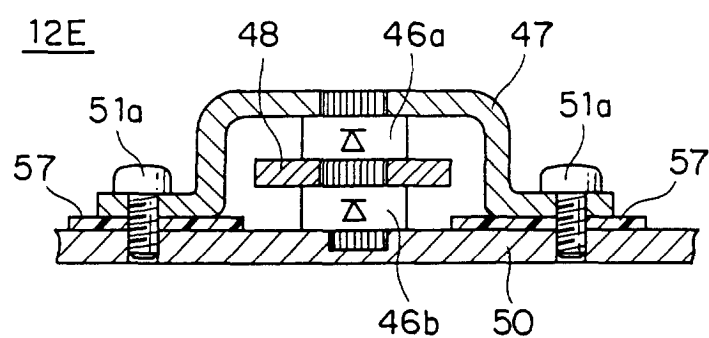
FIG. 35 PRIOR ART
