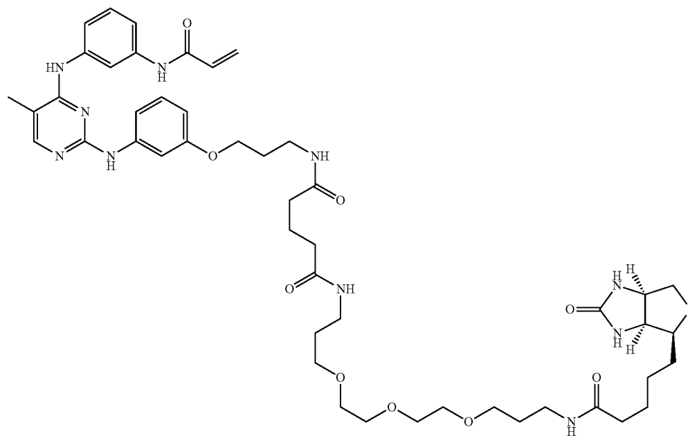
Covalent Probe
