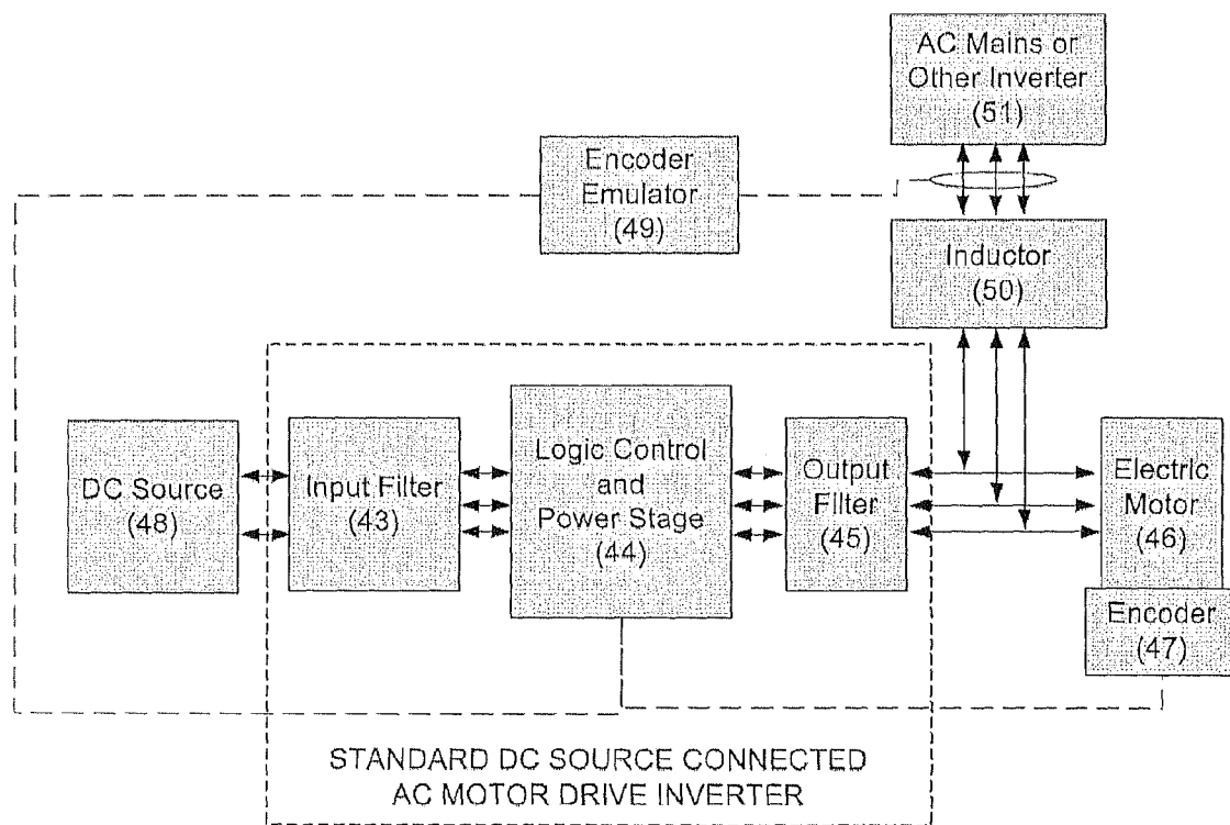
Figure 2C: System of Invention Using Encoder Emulator
