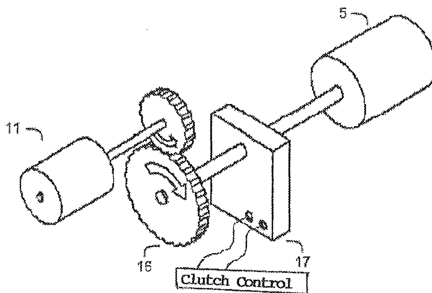
Figure 5: Alternate Motor Coupling Method
