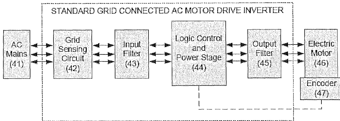
Figure 2A: PRIOR ART Standard Grid Connected AC Motor Drive Inverter
