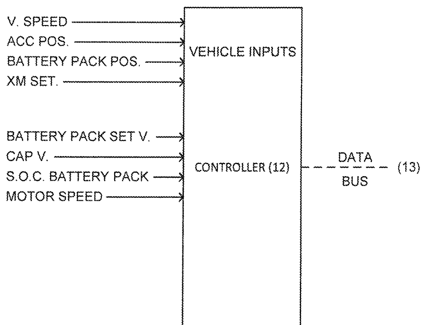
Figure 4: Vehicle Controller
