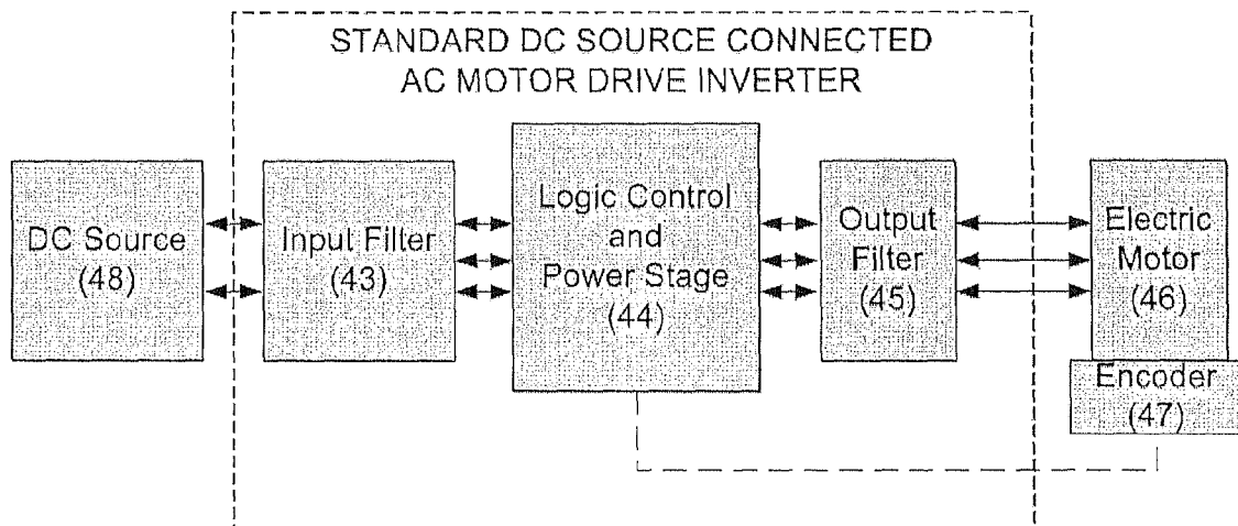
Figure 2B: PRIOR ART Standard DC Source Connected AC Motor Drive Inverter
