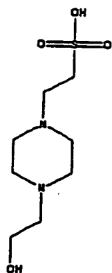
Hepes
