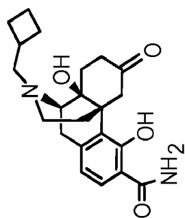
Compound A
