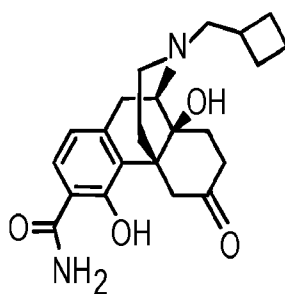
Compound A
