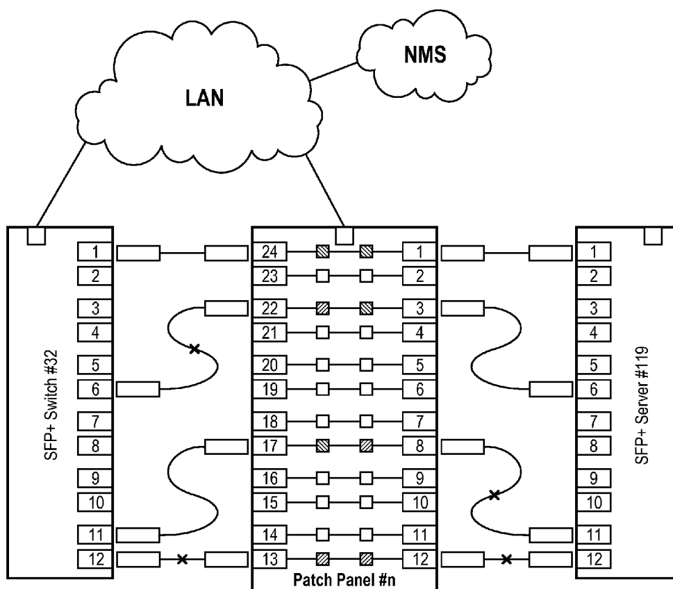
Data Communication Paths that NMS reports
