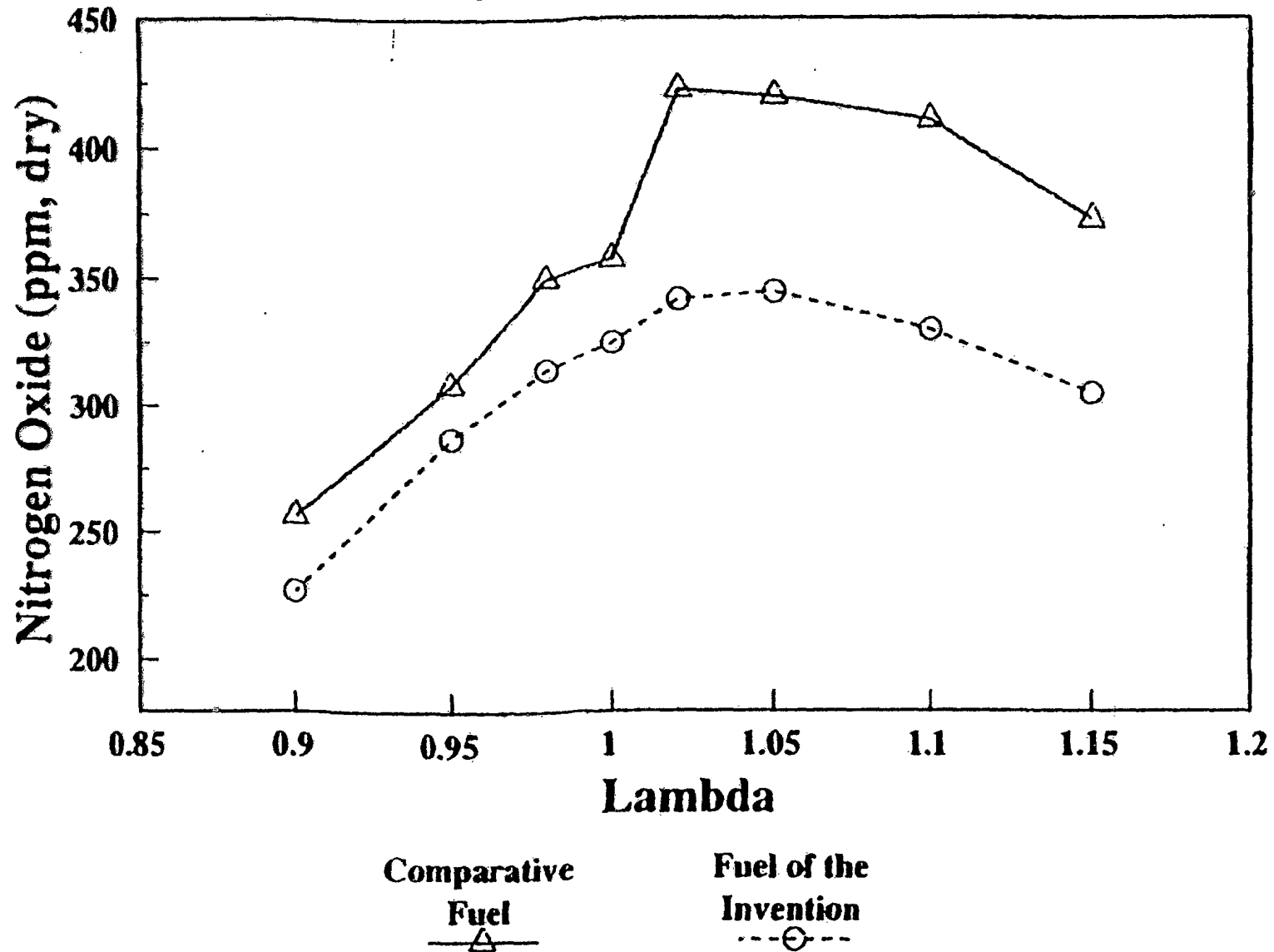
Figure 1. Nitrogen Oxide Exhaust Emissions
