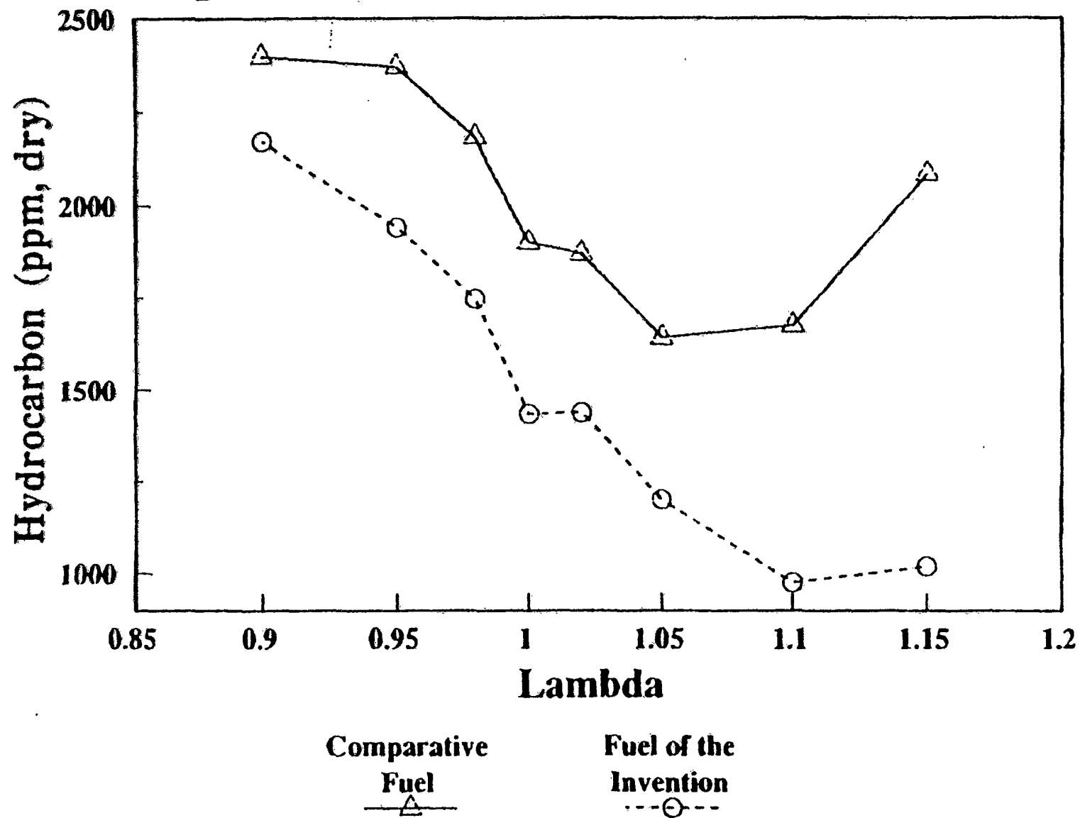
Figure 2. Hydrocarbon Exhaust Emissions
