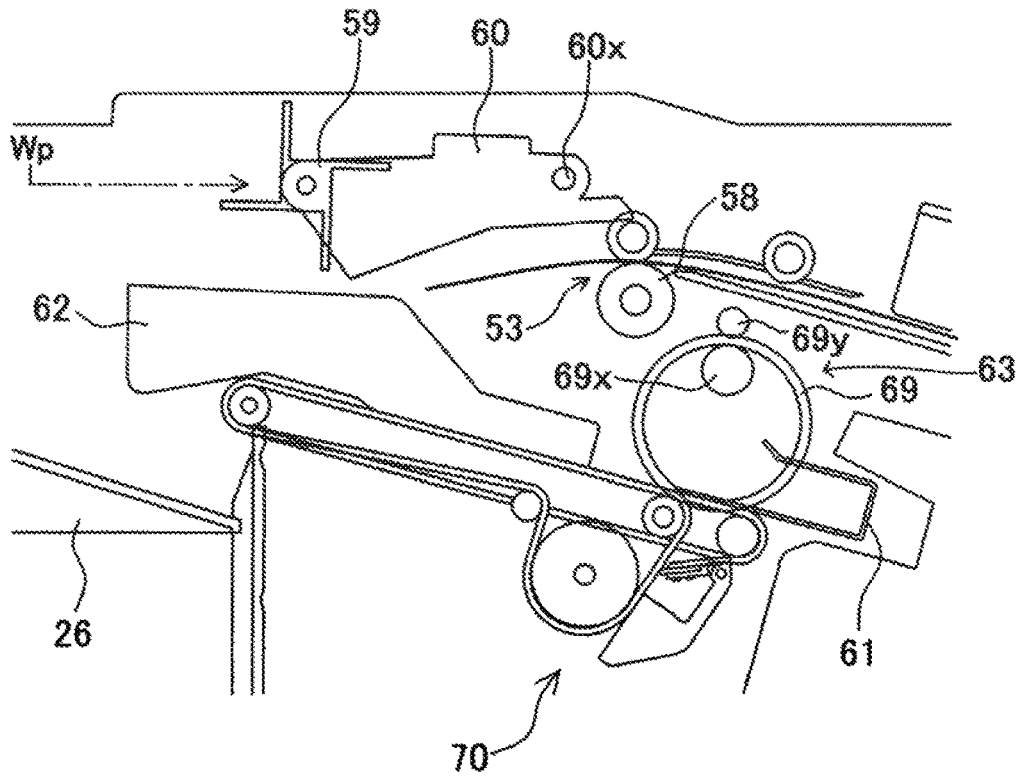
FIG. 4A Paddle elevated position Sheet discharge
