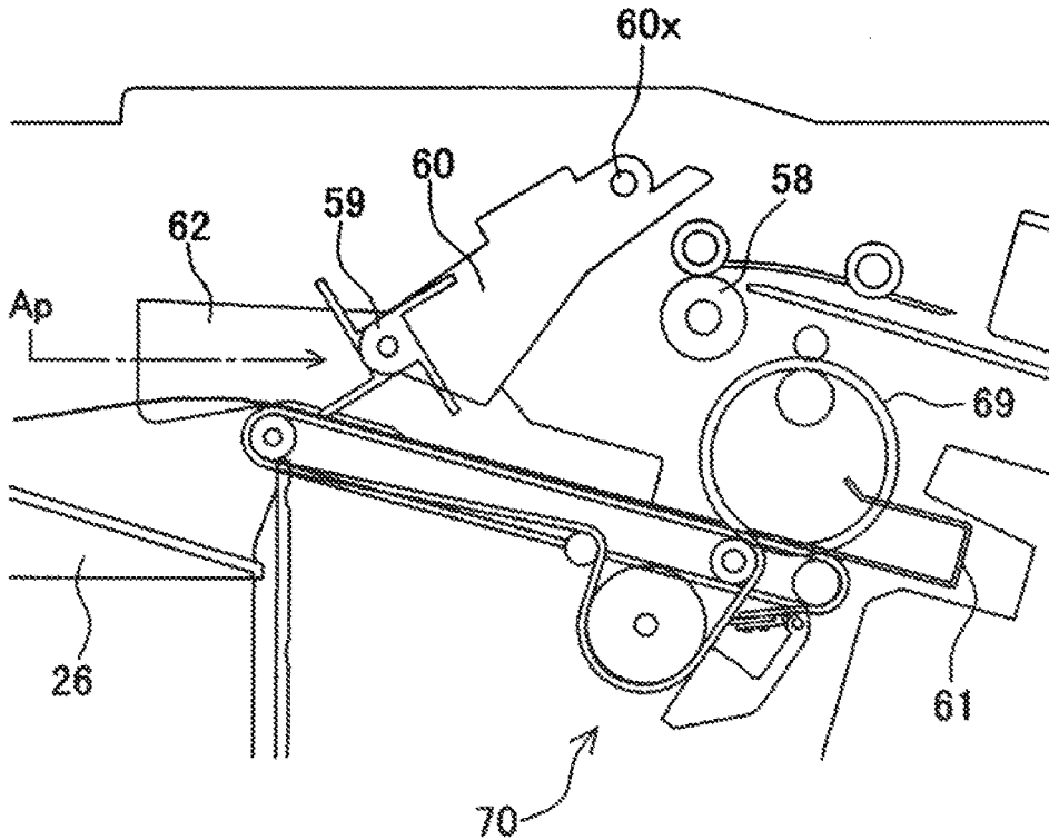
FIG. 4B Paddle lowered position
