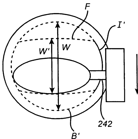
FIG. 22D (PRIOR ART COMPARISON)
