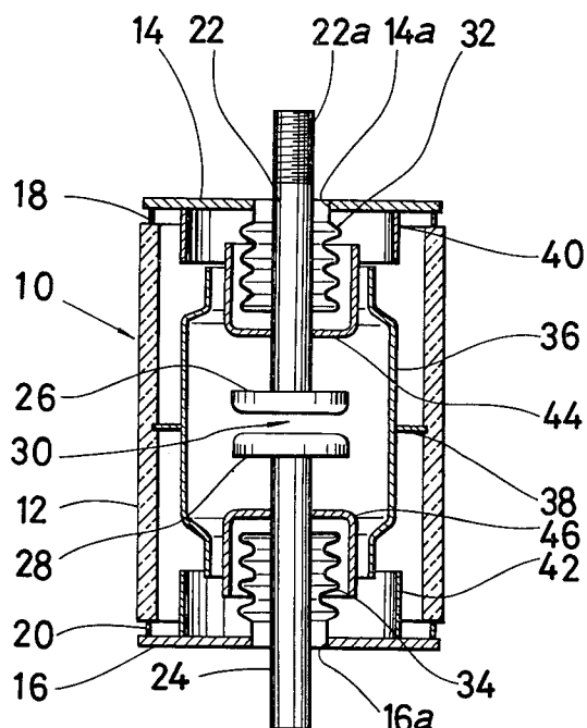
FIG. 1 PRIOR ART
