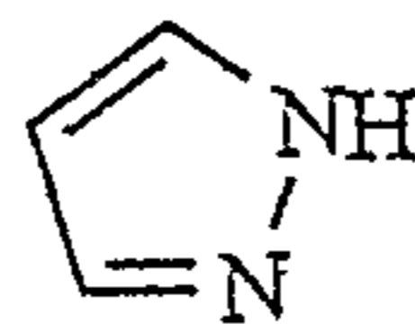
pyrazole
