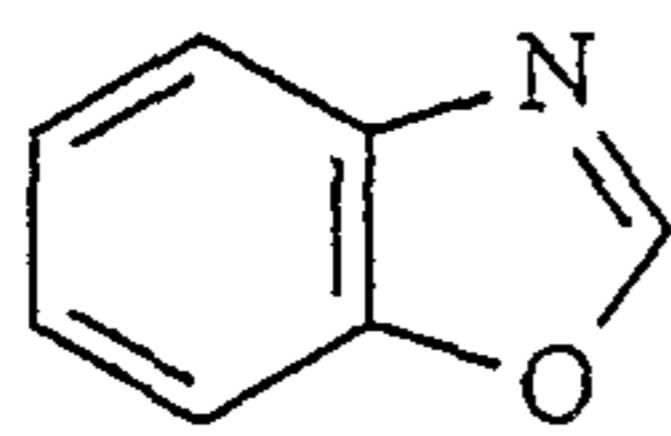
benzoxazole
