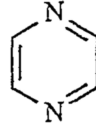
pyrazine
