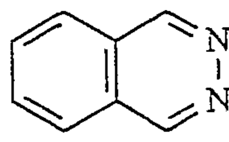
phthalazine
