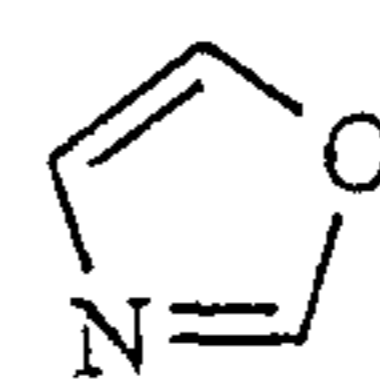
oxazole
