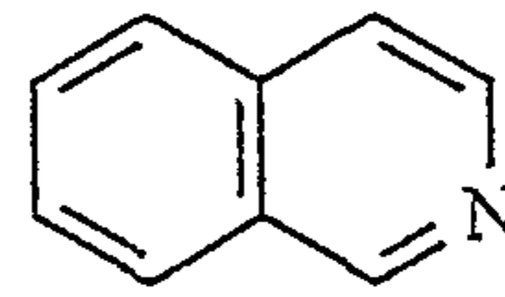
isoquinoline
