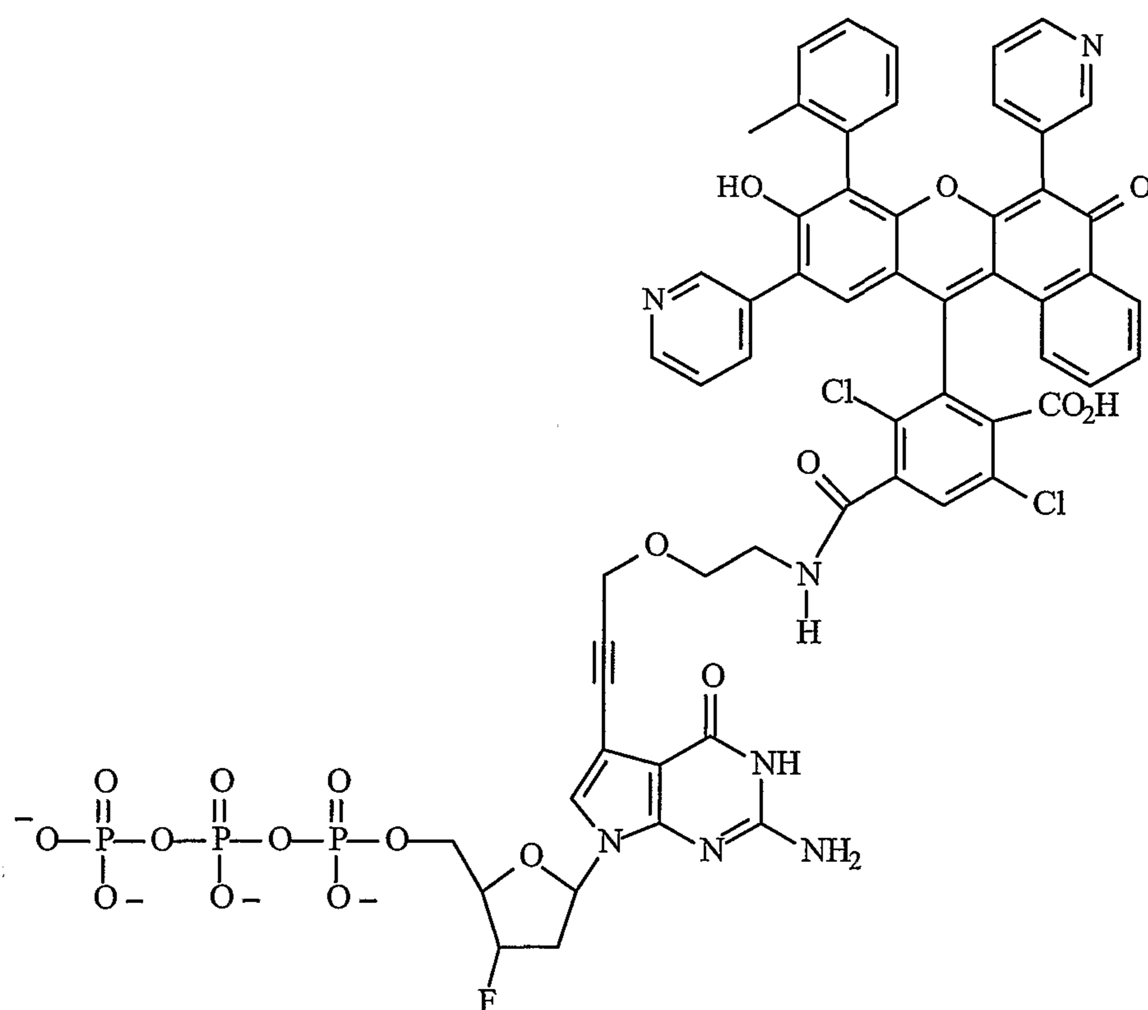
3'FddGTP-EO-13
