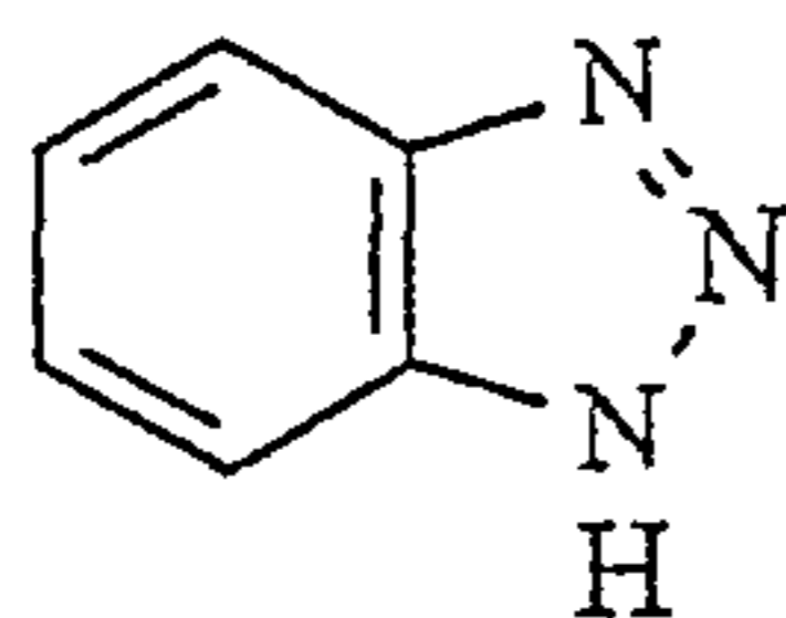
benzotriazole
