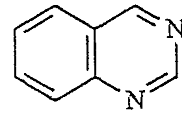
quinazoline
