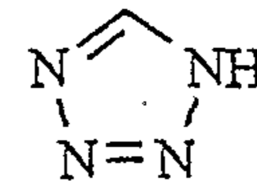
tetrazole
