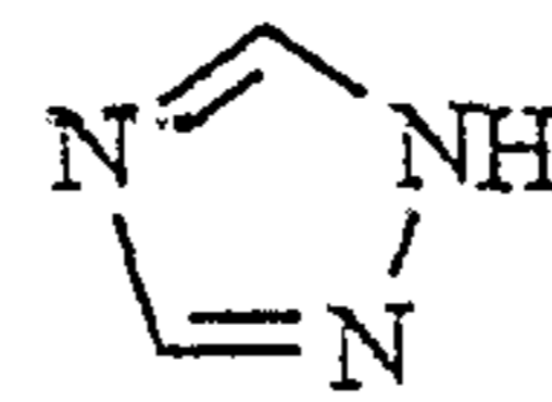
1,2,4-triazole
