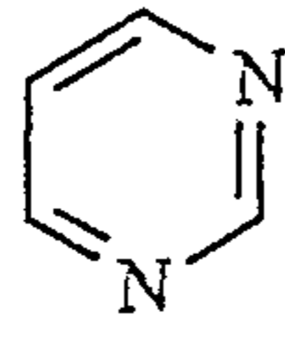
pyrimidine
