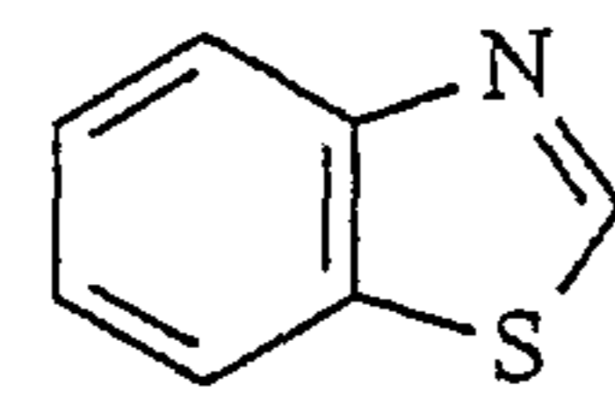
benzothiazole
