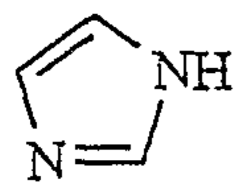
imidazole
