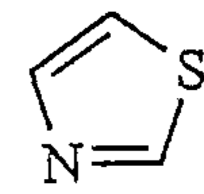
thiazole
