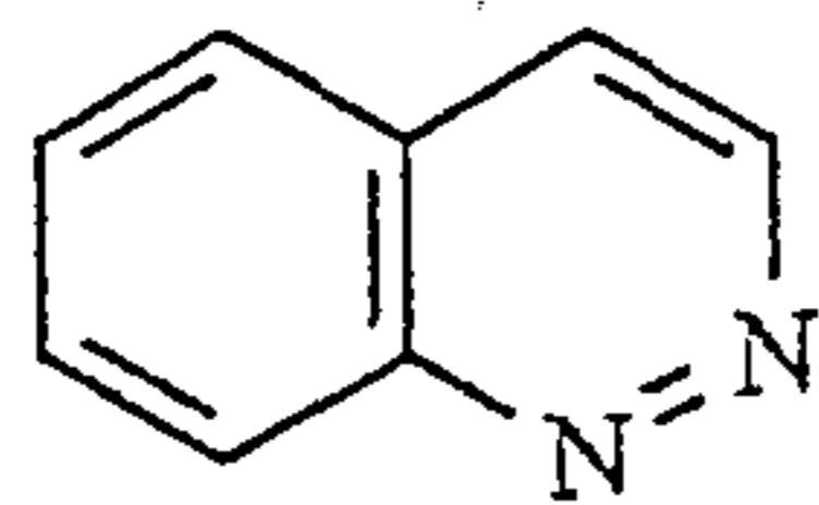
cinnoline
