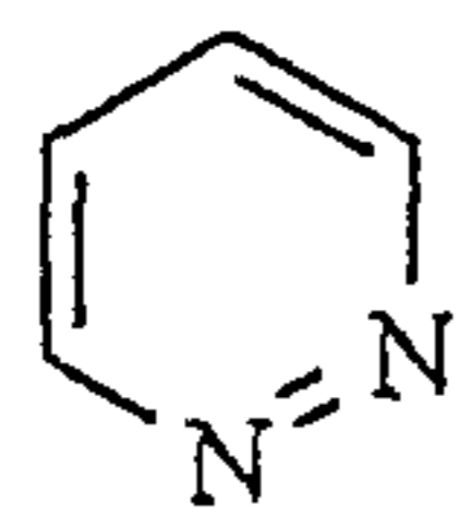
pyridazine
