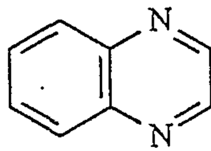
quinoxaline
