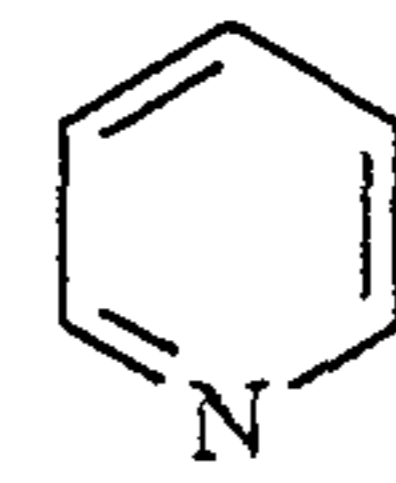
pyridine
