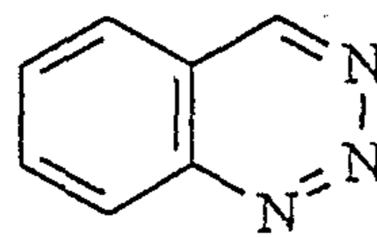
benzotriazine
