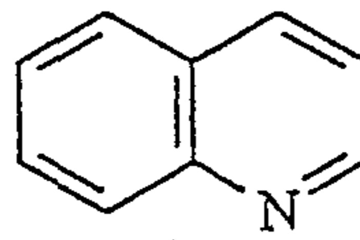
quinoline
