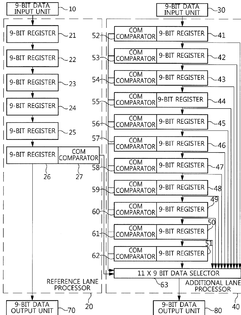
FIG. 1 (PRIOR ART)
