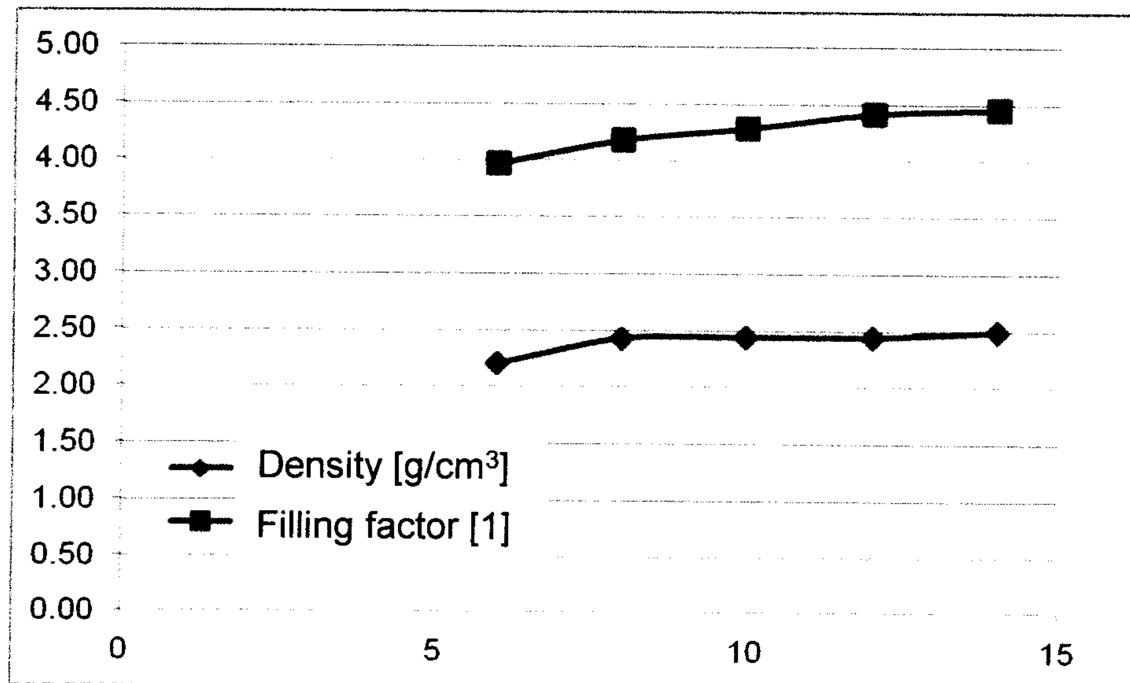
Figure 1. Density and filling factor as a function of the pressing pressure.
