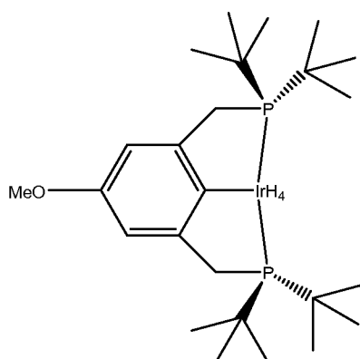
Complex 5: (p-OMe t Bu 4 PCP)IrH 4 ;
