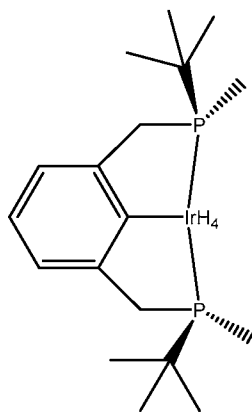
Complex 3: ( t\text{Bu}^2\text{Me}^2\text{PCP} )IrH 4 ;
