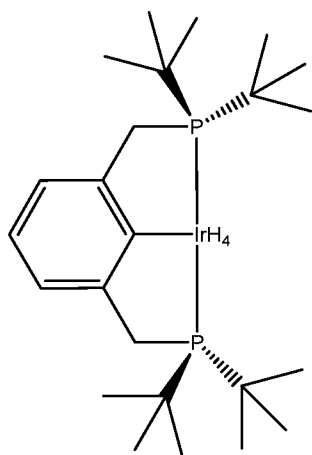
Complex 1: ( t\text{Bu}^4\text{PCP} )IrH 4 ;
