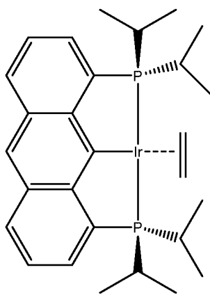
Complex 9: ( i\text{Pr}^4\text{Anthraphos} )Ir(C 2 H 4 )
