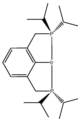
Complex 10: ( i\text{Pr}^4\text{PCP} )Ir;
