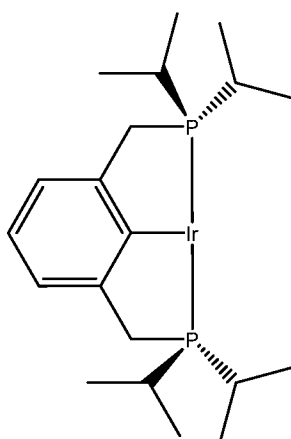
Complex 10: ( i\text{Pr}^4\text{PCP} )Ir;
