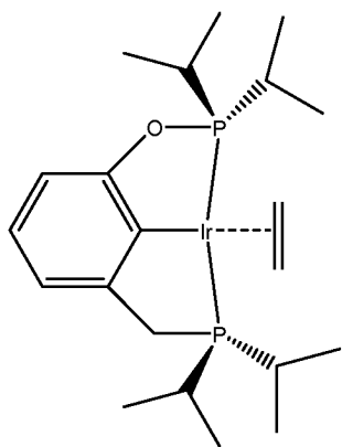
Complex 8: ( i\text{Pr}^4\text{PCOP} )Ir(C 2 H 4 );
