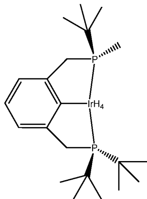
Complex 2: ( t\text{Bu}^3\text{MePCP} )IrH 4 ;
