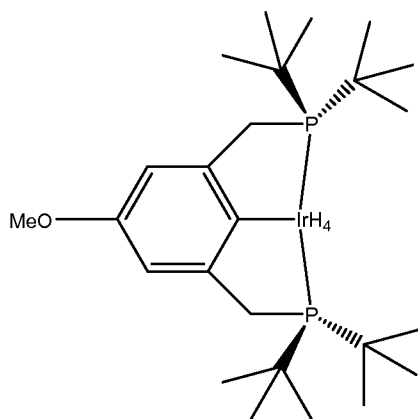
Complex 5: (p-OMe t\text{Bu}^4\text{PCP} )IrH 4 ;
