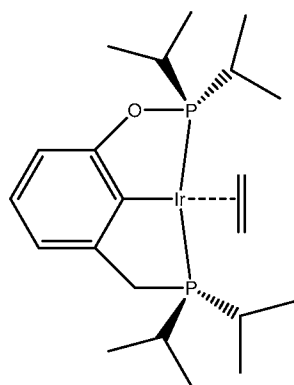
Complex 8: ( i\text{Pr}^4\text{PCOP} )Ir(C 2 H 4 );
