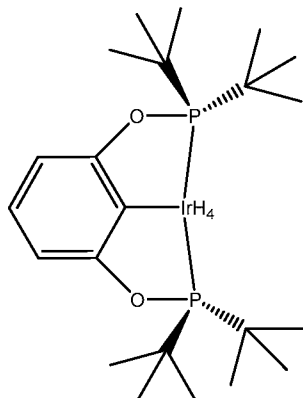
Complex 4: ( t\text{Bu}^4\text{POCOP} )IrH 4 ;
