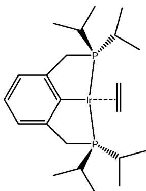
Complex 7: ( i Pr 4 PCP)Ir(C 2 H 4 );
