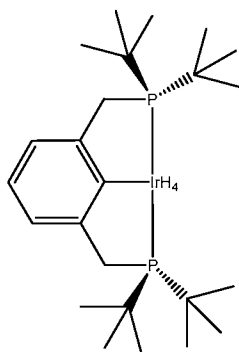
Complex 1: ( t Bu 4 PCP)IrH 4 ;
