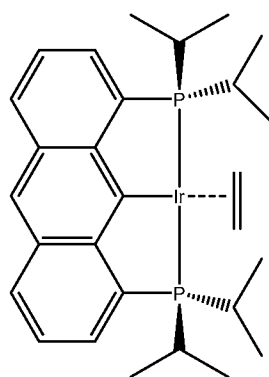
Complex 8: ( i\text{Pr}^4\text{PCOP} )Ir(C 2 H 4 );
