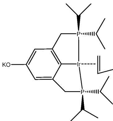
Complex 11: (p-OK- iPr PCP)Ir(C 3 H 6 );
