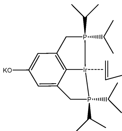
Complex 11: (p-OK- i\text{Pr}^4\text{PCP} )Ir(C 3 H 6 );
