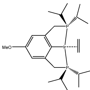
Complex 6: (p-OMe i Pr 4 PCP)Ir(C 2 H 4 );
