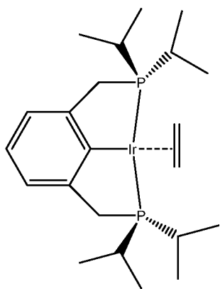
Complex 7: ( i\text{Pr}^4\text{PCP} )Ir(C 2 H 4 );
