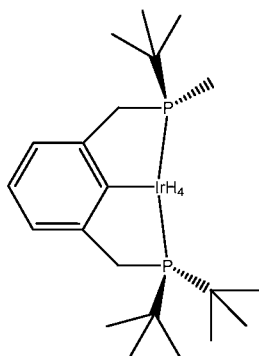
Complex 2: ( t\text{Bu}^3\text{Me}^1\text{PCP} )IrH 4 ;
