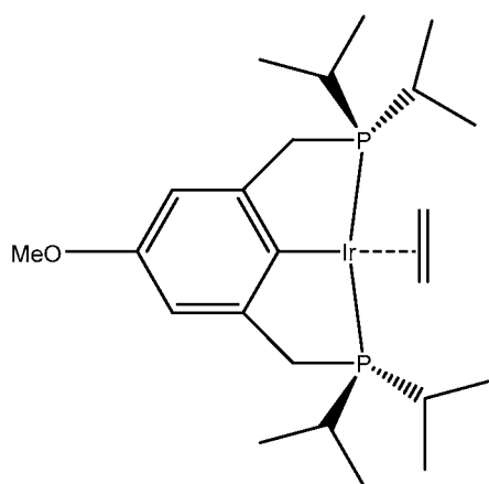
Complex 6: (p-OMe i\text{Pr}^4\text{PCP} )Ir(C 2 H 4 );
