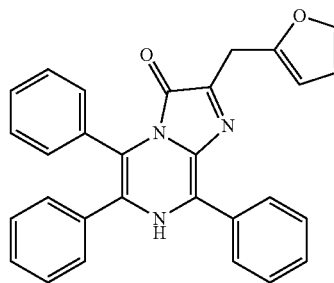
2-(furan-2-ylmethyl)-5,6,8-triphenylimidazo[1,2-a]pyrazin-3(7H)-one
