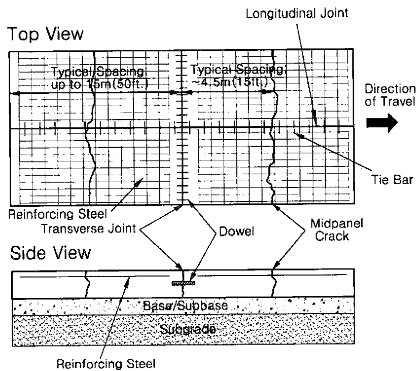
FIG.2 RELATED ART
