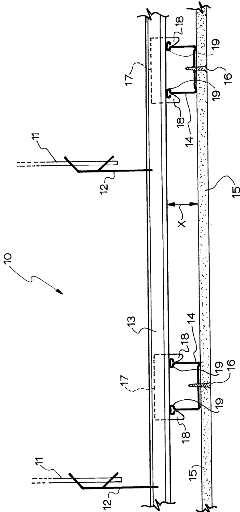
FIG.1 (Prior Art)
