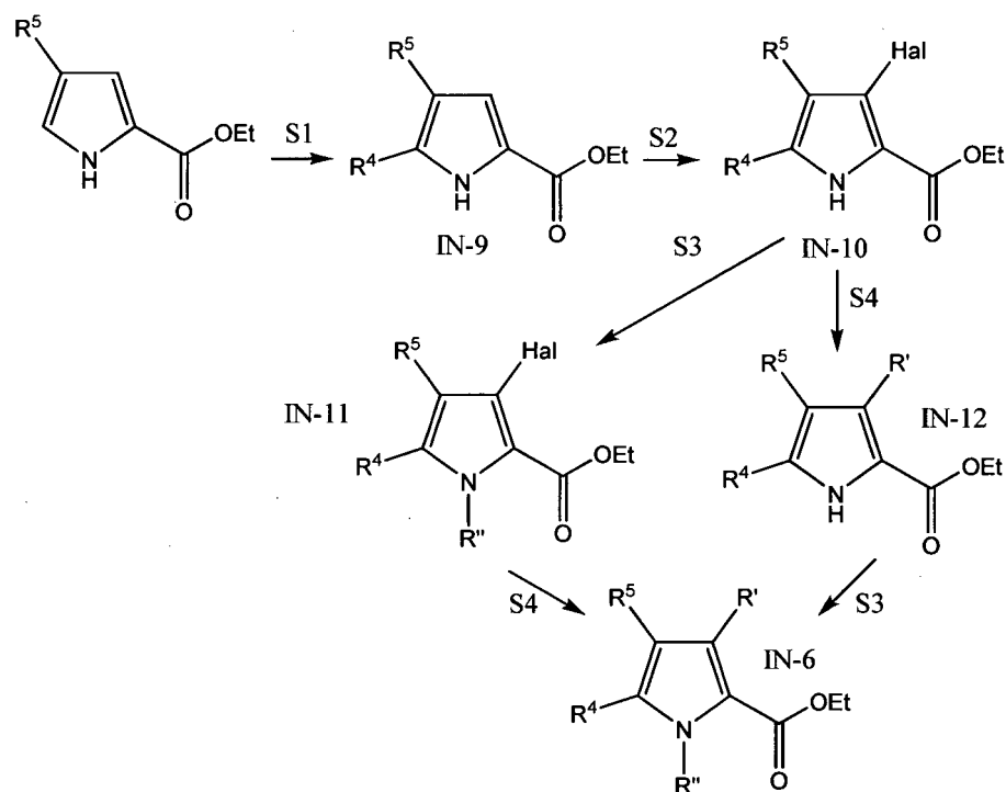
Scheme 4: Alternative synthesis of IN-6.
