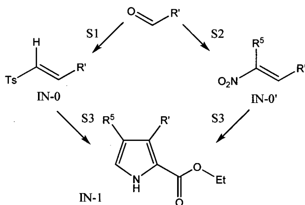
Scheme 1: Preparation of general intermediate IN-1 from aryl aldehydes R'CHO.
