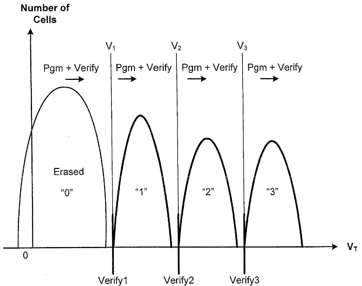
Example of programming a 4-state memory using 3 verify levels
