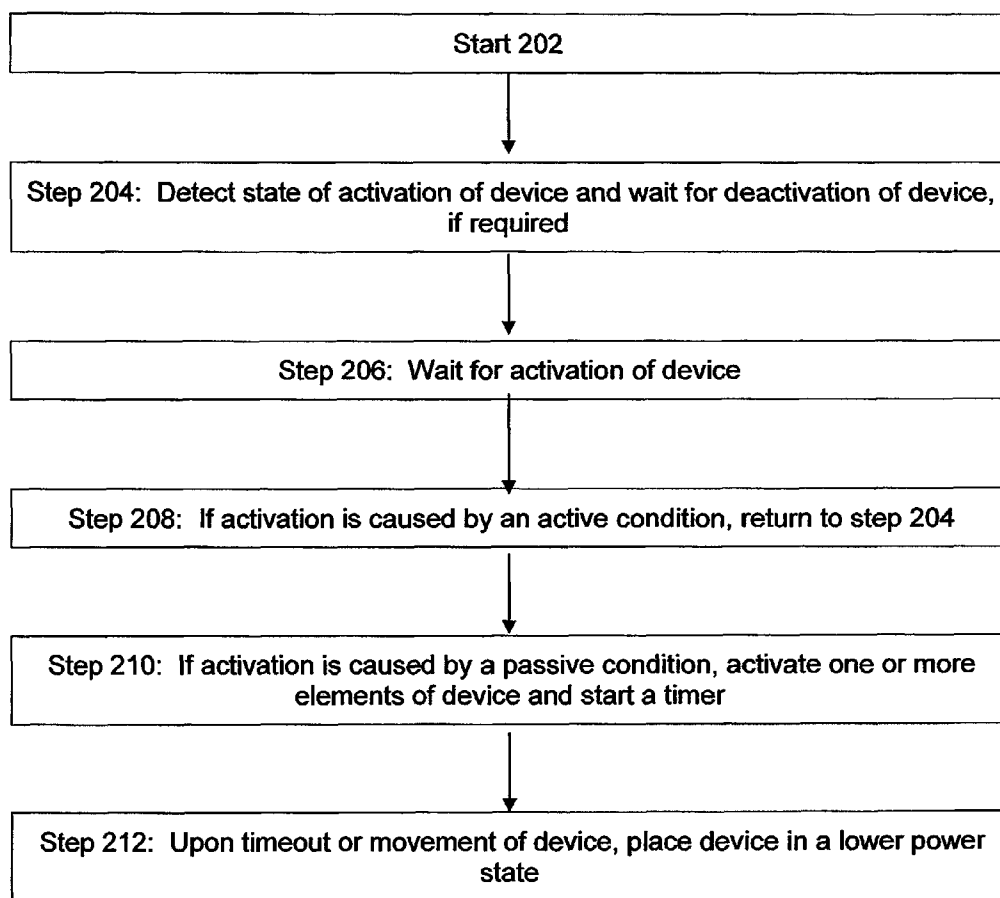
Algorithm 200
