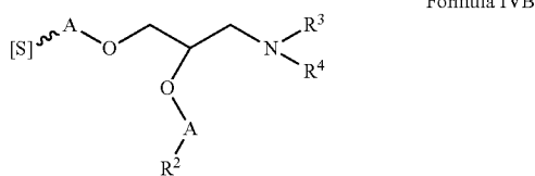
Formula IVB
