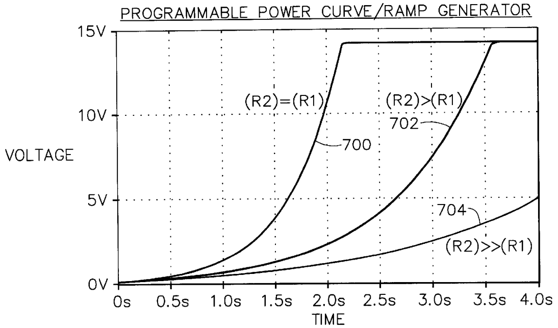
FIG. 7 OUTPUT WAVEFORM
