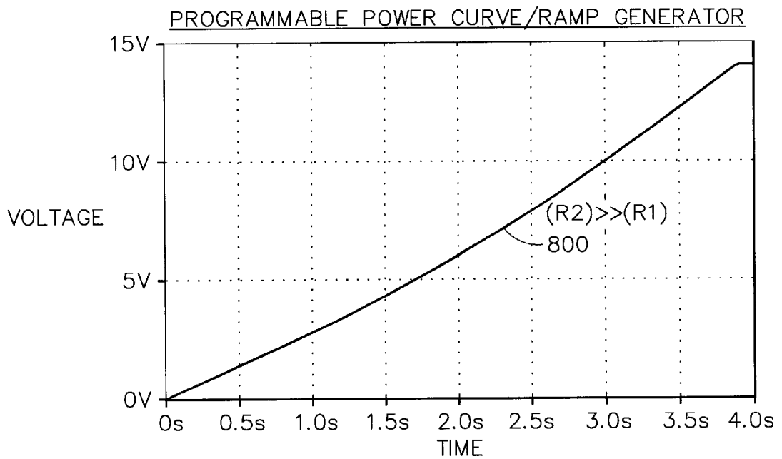
FIG. 8 OUTPUT WAVEFORM
