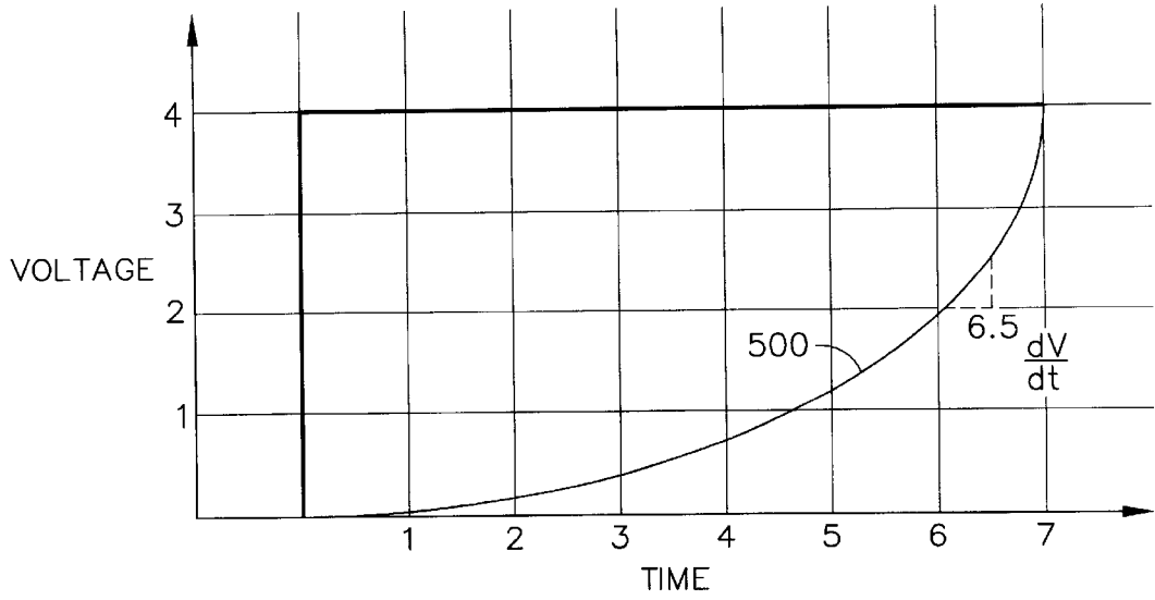
DIVERGENT EXPONENTIAL WAVEFORM
